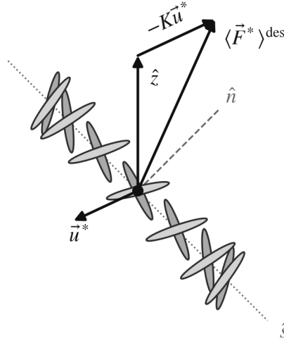
Figure 14: Control-law geometry in the hover use case. The reference velocity is zero (and therefore not drawn): the force demand of Equation 87 composes, tip to tail, the weight compensation \hat{z} with the braking term -K\vec{u}^* opposing the residual drift velocity \vec{u}^* , giving a resultant that supports the weight while arresting the drift. The stroke plane is pinned at \gamma = \gamma^{\text{hover}} = -45^\circ with \psi_1 = \psi_1^{\text{opt}}(0) ; wingbeat overlay as in Figure 10, arrow lengths schematic.
