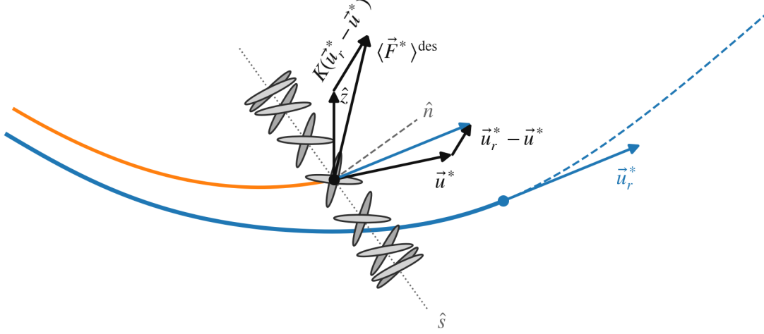
Figure 15: Control-law geometry in the prescribed-trajectory use case. The reference point (dot) travels along the prescribed path (in color, solid where already traveled, dashed ahead) with velocity \vec{u}_r^* , the path tangent scaled by the speed schedule. The body is not constrained to the path: with no position feedback it trails the reference, cutting slightly inside the bend, and its velocity \vec{u}^* lags the leveling-off of the path. The reference velocity is copied at the body (in color) to close the velocity triangle, and the force demand of Equation 87 composes, tip to tail, the weight compensation \hat{z} with the amplified error K(\vec{u}_r^* - \vec{u}^*) . Wingbeat overlay as in Figure 16, at the blended stroke-plane angle for the drawn J \approx 0.2 ; arrow lengths are schematic.
