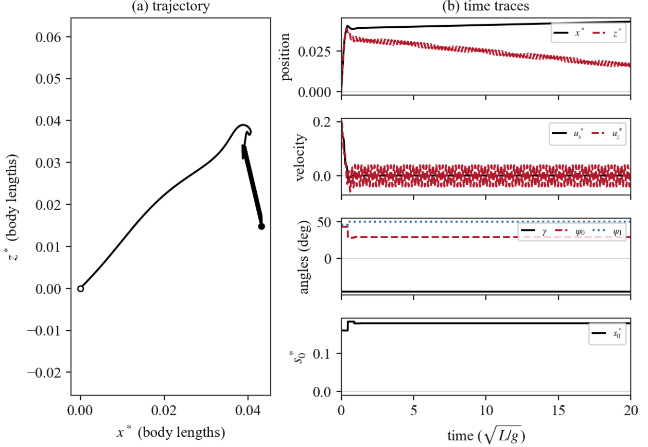
Figure 17: Hover hold under the velocity law (Equation 87, K = 2.7 ). The velocity perturbation is eliminated within about one time unit. The position offset accumulated meanwhile (about 0.05 body lengths) is never corrected—there is no position feedback—and some slow residual drift remains, but the body settles into a clean hover about the settled point.
