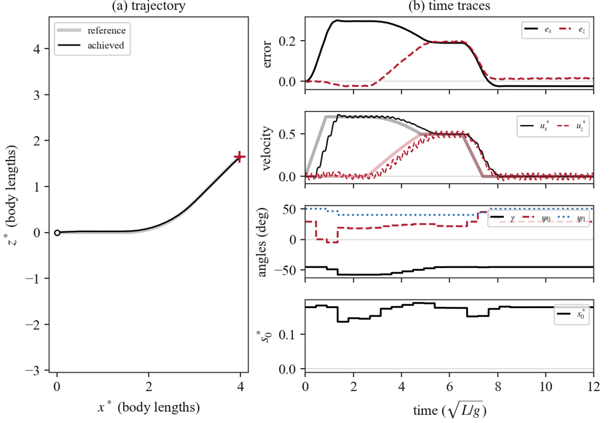
Figure 18: Prescribed trajectory under the velocity law ( K = 2.7 ): the body follows the commanded velocity with a first-order lag, trailing the reference point by |\vec{u}_r^*|/K \approx 0.26 body lengths through the cruise; the deceleration ramp lets it catch up near the end. Position drift is not corrected, but the achieved path stays close to the reference.
