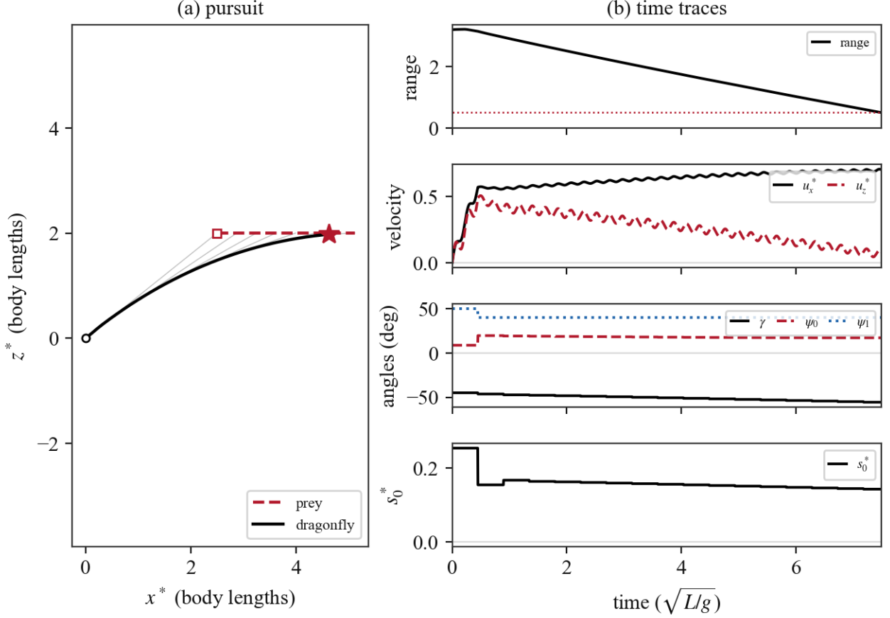
Figure 19: Prey pursuit. (a) The line-of-sight command produces the classical pure-pursuit tail chase, with capture at t^* \approx 7.5 (star). (b) The body accelerates to the commanded closing speed ( J \approx 0.2 ). \gamma leans from \gamma^{\text{hover}} toward alignment with the flight direction, \psi_1 follows its slaved schedule (Equation 91), and (s_0^*, \psi_0) trim the force demand.
