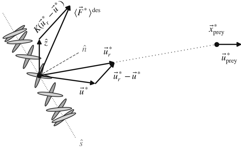
Figure 16: Control-law geometry in the prey pursuit use case. The prey is detected at the line-of-sight bearing \hat{r} (sparse dots), and the reference velocity \vec{u}_r^* = u_{\text{cmd}}^* \hat{r} (Equation 88) points along it, while the body velocity \vec{u}^* lags behind (tail chase, the prey moving along +\hat{x} ). The velocity error \vec{u}_r^* - \vec{u}^* closes the velocity triangle, and the force demand of Equation 87 composes, tip to tail, the weight compensation \hat{z} with the amplified error K(\vec{u}_r^* - \vec{u}^*) . The wingbeat overlay is drawn as in Figure 10, at the blended stroke-plane angle of Equation 90 for the drawn J \approx 0.2 ( \gamma \approx -60^\circ , \psi_1 = \psi_1^{\text{opt}}(J) ); velocity and force arrow lengths are schematic.
