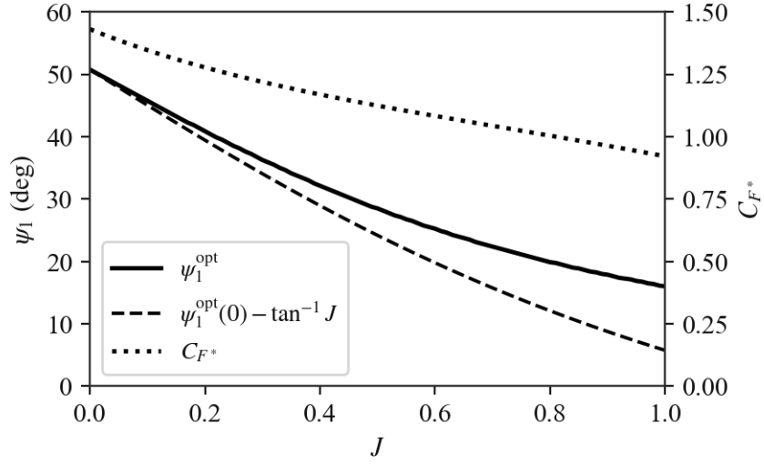
Figure 12: Pitch amplitude \psi_1^{\text{opt}} and force coefficient C_{F^*} of the continued hover optimum (the point tracked in Figure 11) as functions of advance ratio J . The dashed line is the approximation \psi_1^{\text{opt}}(0) - \tan^{-1} J , which holds the midstroke \alpha constant as J increases.
