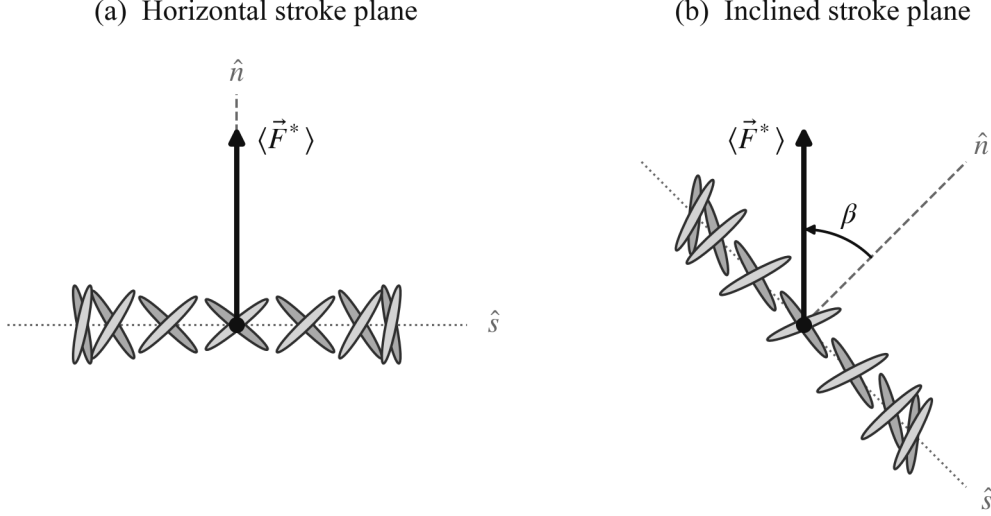
Figure 10: Hover at (a) a horizontal stroke plane and (b) an inclined stroke plane (drawn here with \gamma < 0 ). The wing is drawn over one full wingbeat at equal time increments, with the -\hat{s} half-stroke behind, in darker grey, and the +\hat{s} half-stroke in front. In (a), the reference pitch kinematics ( \psi_0 = 0^\circ ) set the mean force \langle \vec{F}^* \rangle vertically along \hat{n} . In (b), the mean force remains vertical while \hat{n} is tilted because \psi_0^{\text{hover}} is trimmed to bias \langle \vec{F}^* \rangle by \beta = -\gamma^{\text{hover}} using the inverse of Equation 49.
