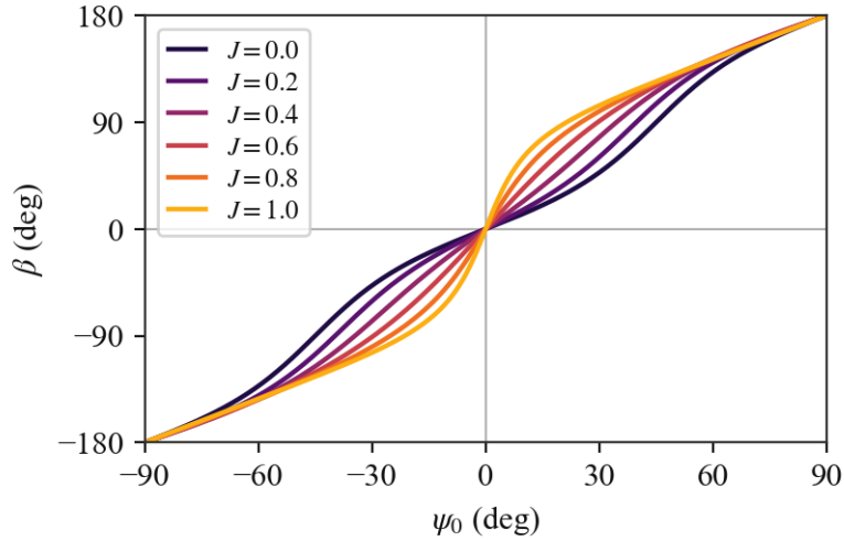
Figure 13: Effect of \psi_0 on the force direction angle \beta for increasing advance ratio J , at \delta_0 = 90^\circ and with \psi_1 = \psi_1^{\text{opt}}(J) . Unlike in the hover case, \beta depends on \psi_1 when J > 0 .
