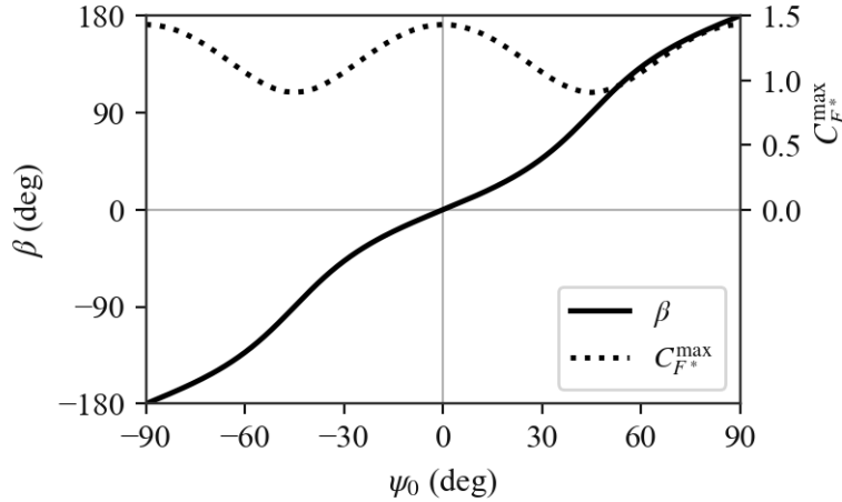
Figure 9: Effect of \psi_0 on force direction angle \beta and force coefficient C_{F^*} .
