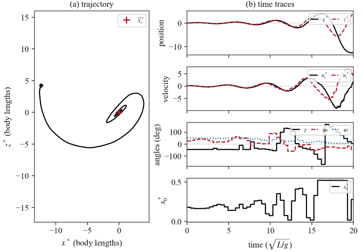
Figure 14: Hover hold with position feedback only ( K_d = 0 ). The oscillation about \vec{x}_r^* is not damped, and the phase lag of the once-per-wingbeat control update makes it grow. Once the position error exceeds the hover pin radius, \gamma and \psi_1 resume scheduling and the trim saturates.
