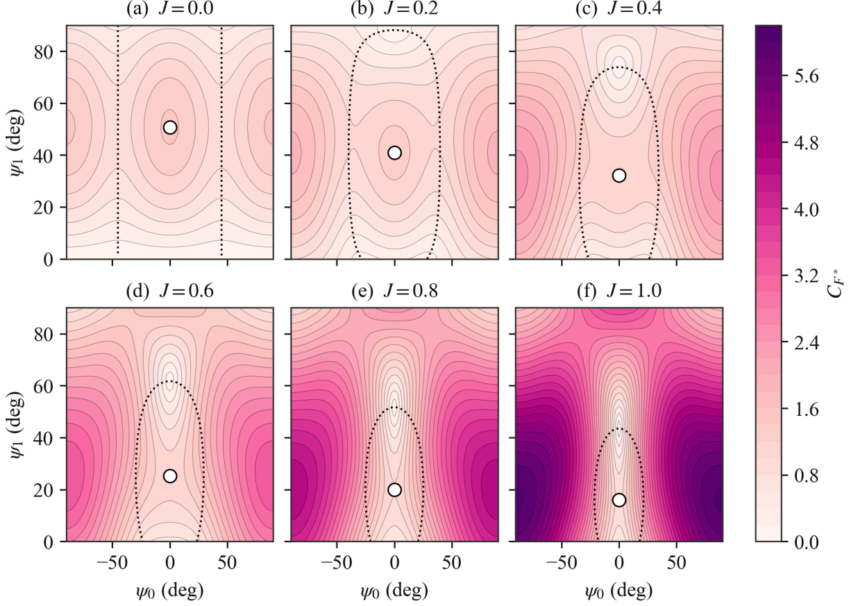
Figure 11: Force coefficient C_{F^*} over the pitch plane (\psi_0, \psi_1) at \delta_0 = 90^\circ , for increasing advance ratio J . White dots track the hover optimum as it moves with J . It remains on the \psi_0 = 0^\circ axis by symmetry while \psi_1 decreases, and it turns from a local maximum into a saddle point. The global maximum sits at large |\psi_0| , where the force is dominated by drag from the normal inflow and points along -\hat{n} . The dotted contour marks C_{F_n^*} = 0 , the boundary between propulsive ( +\hat{n} ) and braking ( -\hat{n} ) mean force.
