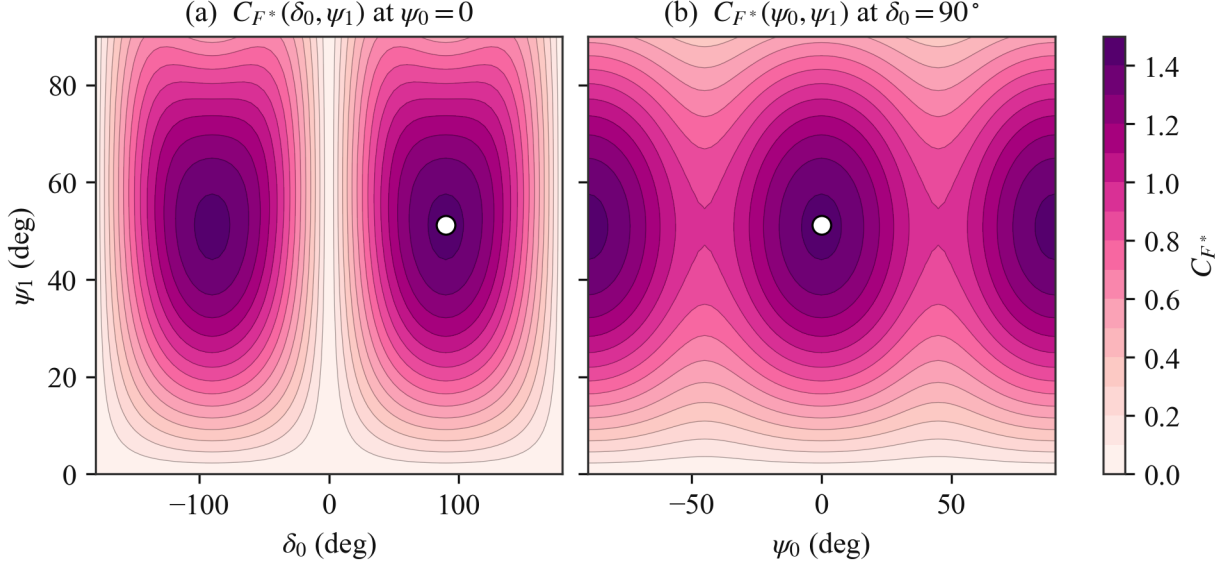
Figure 8: Dependence of C_{F^*} on pitch parameters at zero body velocity. Maximum shown as white dots.
