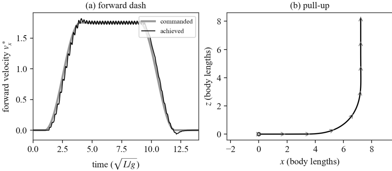
Figure 13: Closed-loop maneuvers (unsteady simulation, control updated once per wingbeat). (a) Forward dash: commanded vs. achieved forward velocity through accelerate–cruise–decelerate. (b) Pull-up: the sagittal-plane path, with body-velocity arrows rotating from horizontal to vertical.
