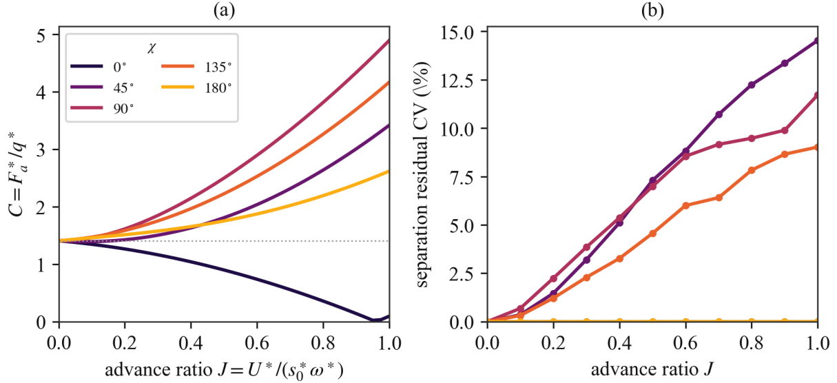
Figure 7: Survival of the F_a^* = q^* C_{F^*} separation at nonzero body velocity. (a) C_{F^*} at nominal pitch as a function of advance ratio for several inflow directions \chi . (b) Separation residual, evaluated as the coefficient of variation of F_a^*/q^* over random draws of the morphological and wingbeat parameters at fixed pitch.
