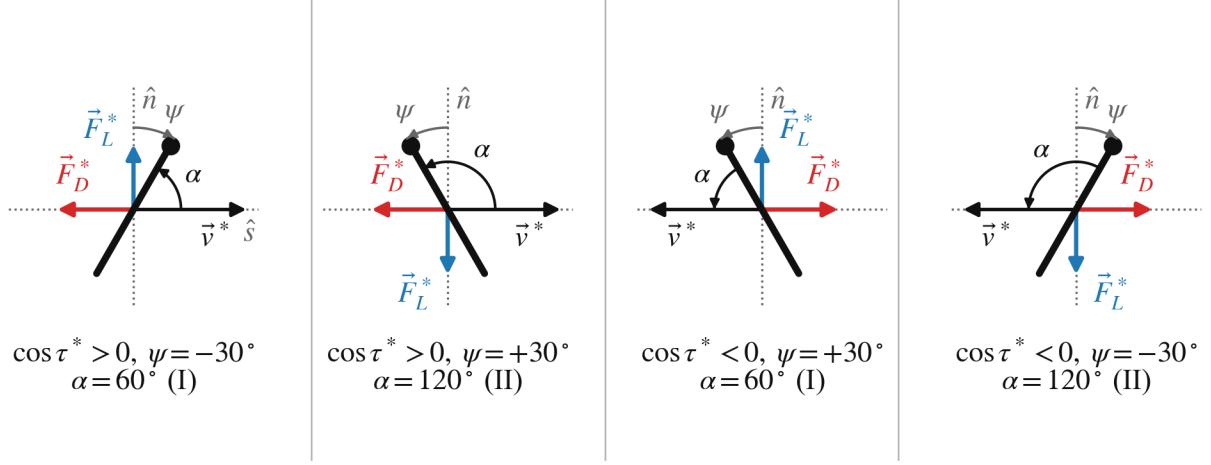
Figure 1: Verification of the hover ( J = 0 ) angle-of-attack expression (Equation 29) for the four sign combinations of (\cos \tau^*, \psi) .
