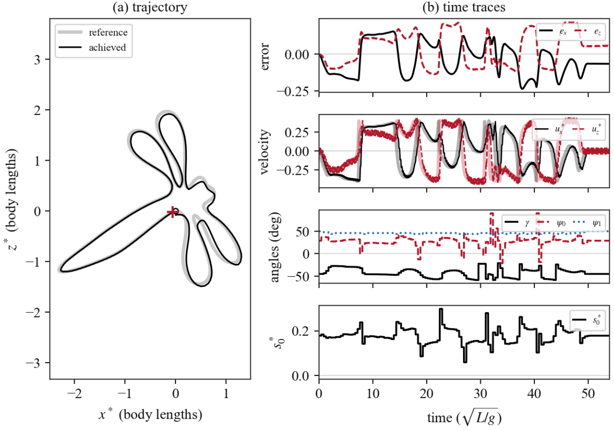
Figure 19: Freehand trajectory under the velocity law ( K = 2.7 , cruise 0.4): a hand-drawn closed course tracing a dragonfly. The body stays within 0.27 body lengths of the reference point throughout and closes the course with a final offset of 0.09.
