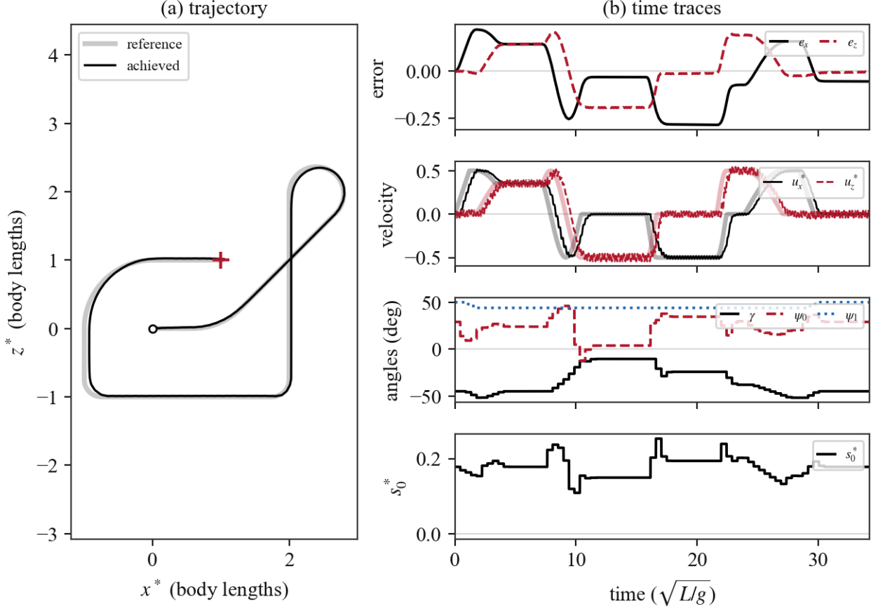
Figure 18: Prescribed trajectory under the velocity law ( K = 2.7 ): the body follows the commanded velocity with a first-order lag, trailing the reference point by |\vec{u}_r^*|/K \approx 0.19 body lengths through the cruise and cutting slightly inside the sharp corners, with the tracking error peaking at 0.28. Position drift is not corrected, but the achieved path stays close to the course throughout—including the loop and the descent—and the body settles next to the course endpoint (final offset 0.06).
