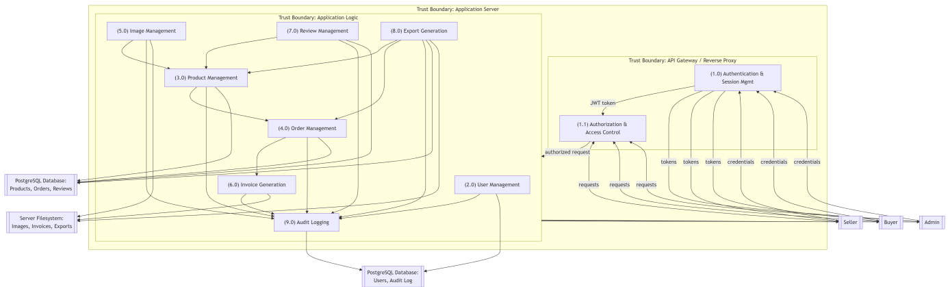
Figure 6: DFD Level 1
