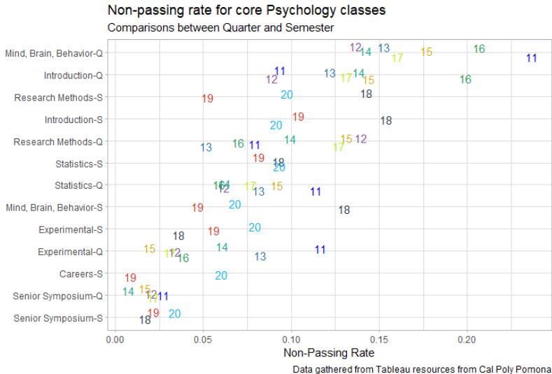
Figure 4: non_passing_rate
