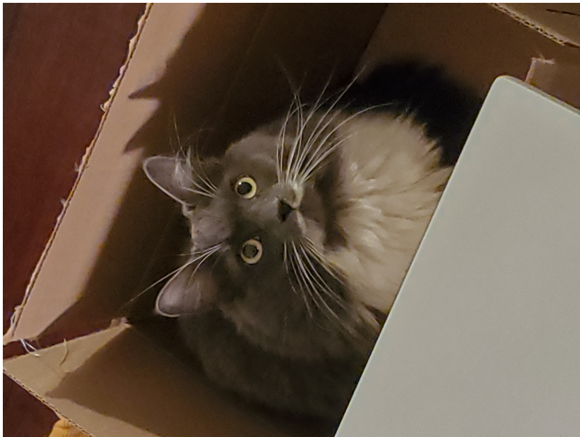
Figure 3: lucy
