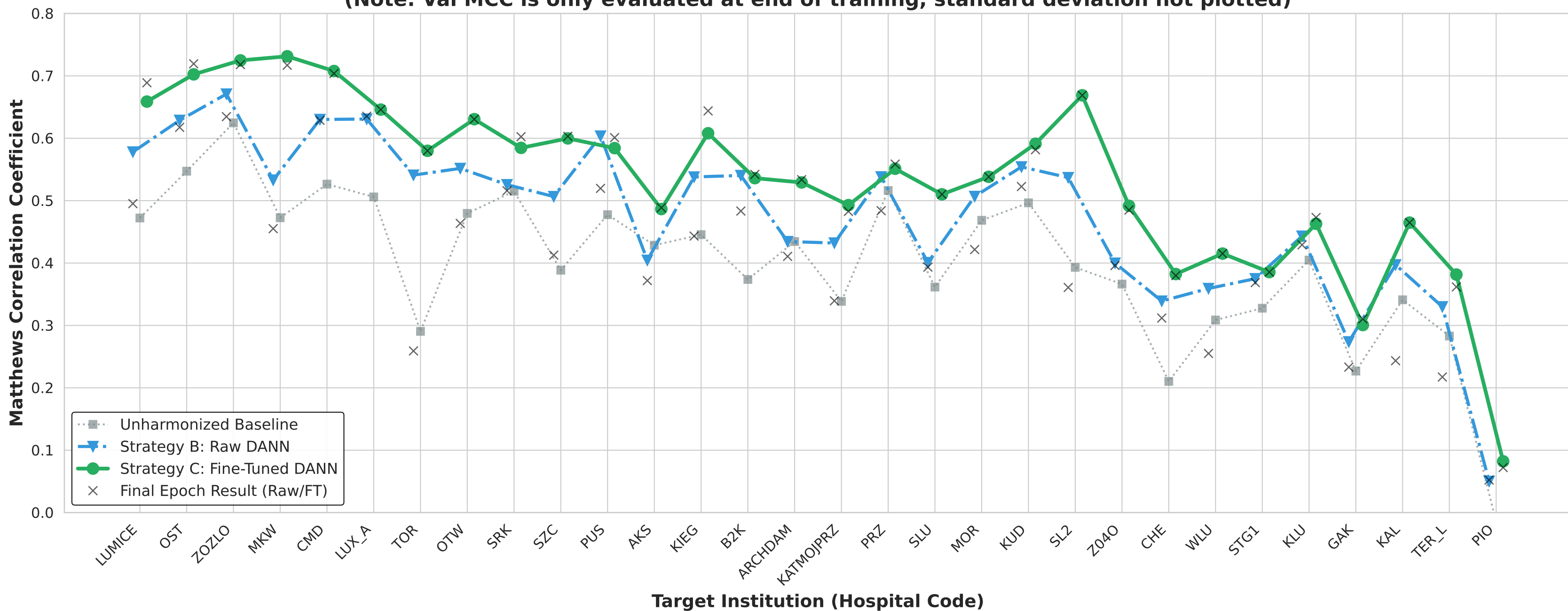
Pathology Classification Performance (MCC): Baseline vs Raw DANN vs Fine-Tuned DANN (Note: Val MCC is only evaluated at end of training, standard deviation not plotted)
