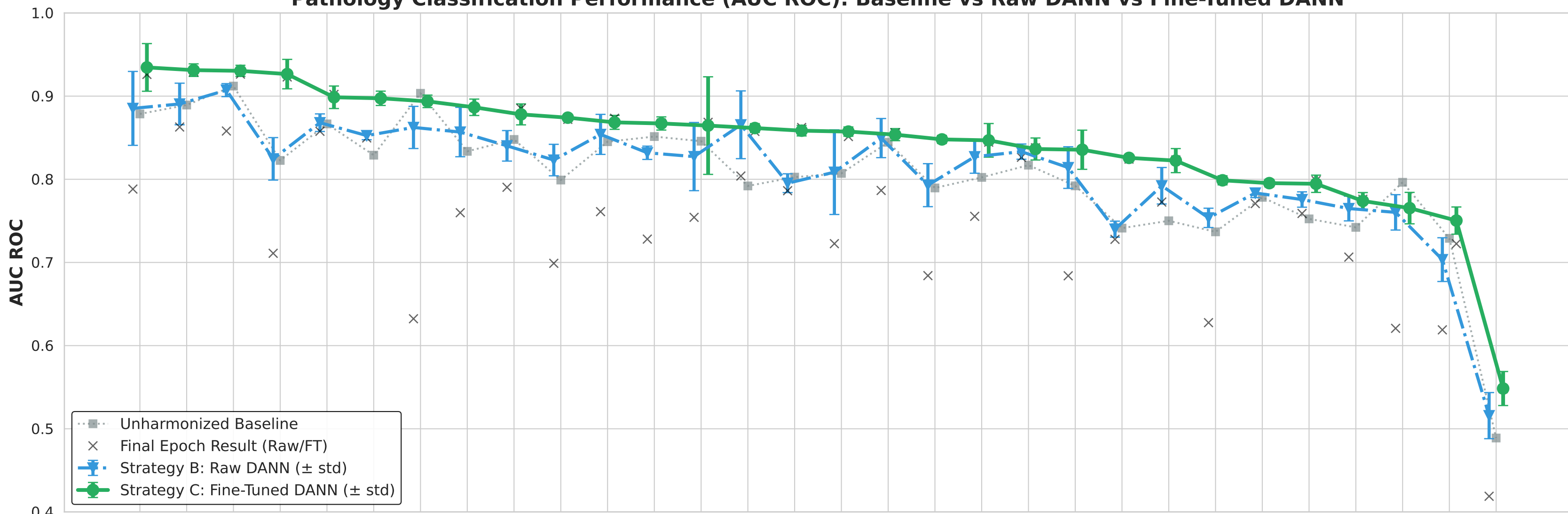
Pathology Classification Performance (AUC ROC): Baseline vs Raw DANN vs Fine-Tuned DANN
