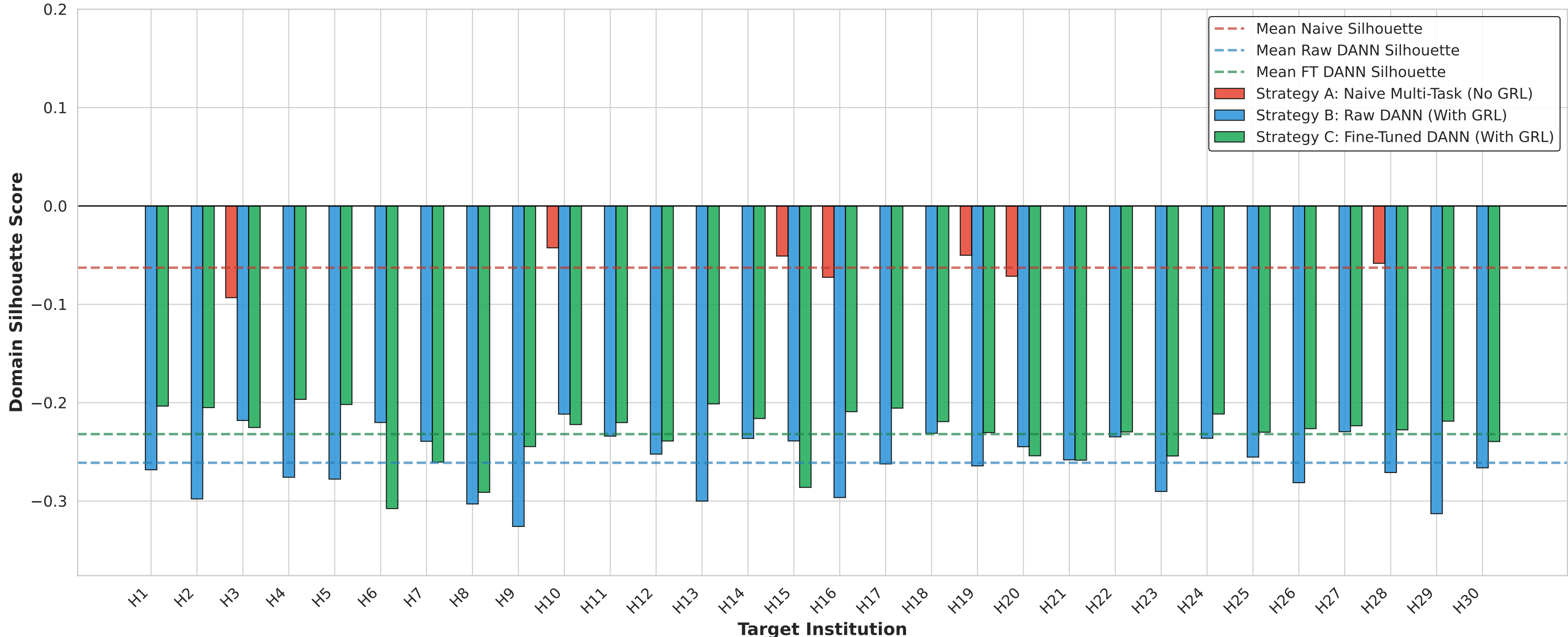
Residual Site Effect: Domain Silhouette Score of Latent Representations
