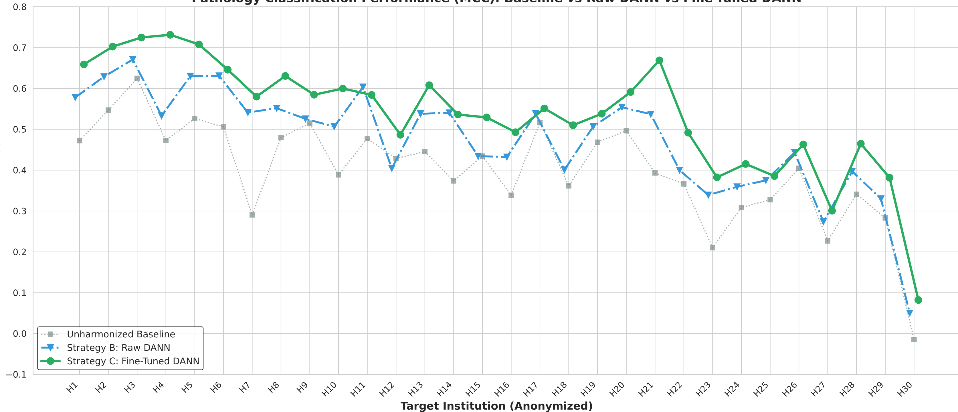
Pathology Classification Performance (MCC): Baseline vs Raw DANN vs Fine-Tuned DANN
