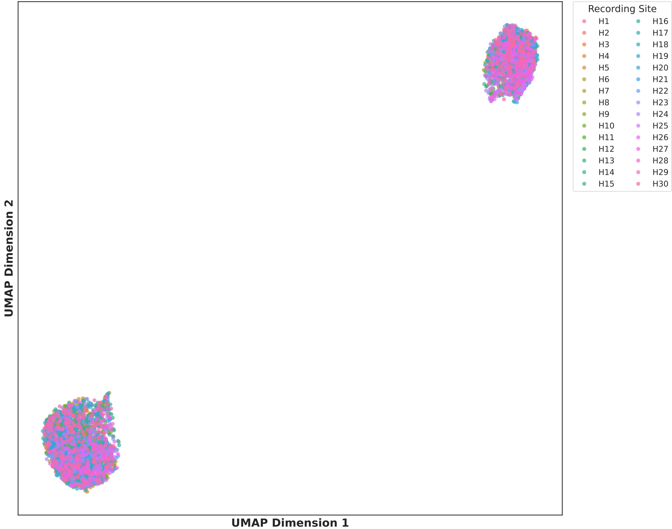
UMAP Projection of Fine-Tuned DANN Latent Space ( \mathbf{f} \in \mathbb{R}^{288} )
