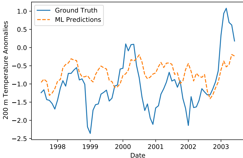
Predicted and True Ocean Temperature Anomalies at 6 Month Lead Time. Corr: 0.44
