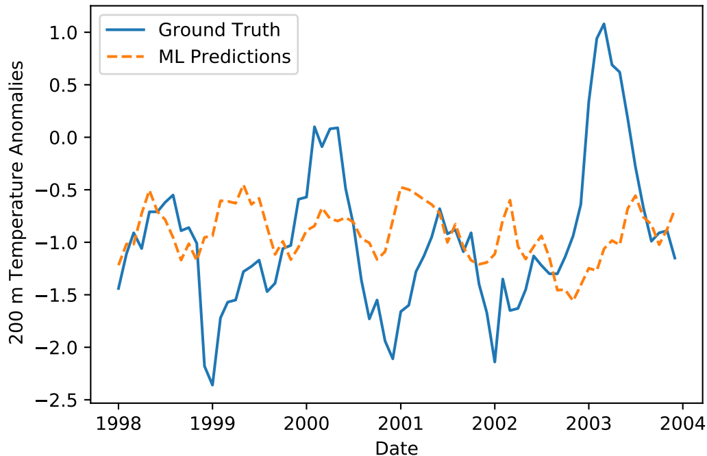
Predicted and True Ocean Temperature Anomalies at 12 Month Lead Time. Corr: -0.06
