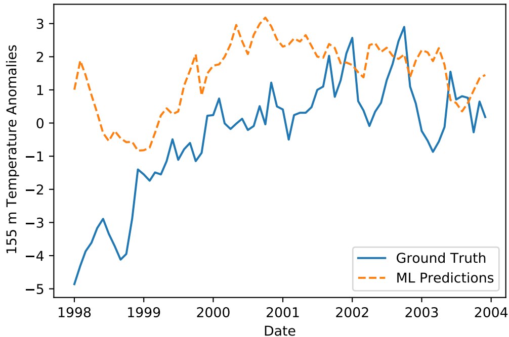
Predicted and True Ocean Temperature Anomalies at 12 Month Lead Time. Corr: 0.57
