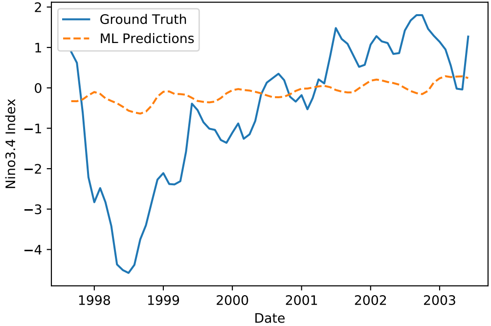
twolayerCNN_1980-01-01_1995-12-31 Predictions. Corr: 0.674099. RMSE: 1.639397.
