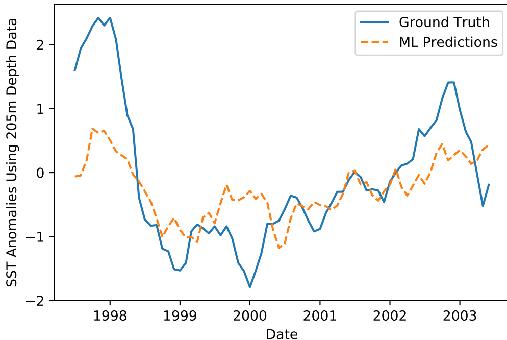
Predicted and True Ocean Temperature Anomalies at 6 Month Lead Time. Corr: 0.78
