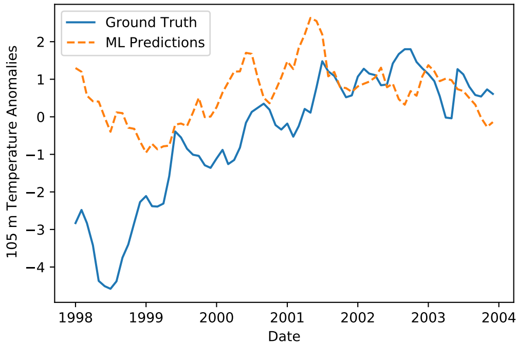
Predicted and True Ocean Temperature Anomalies at 12 Month Lead Time. Corr: 0.46
