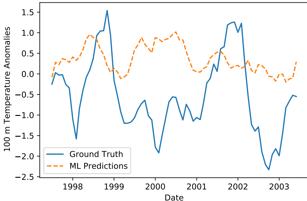
Predicted and True Ocean Temperature Anomalies at 6 Month Lead Time. Corr: 0.11
