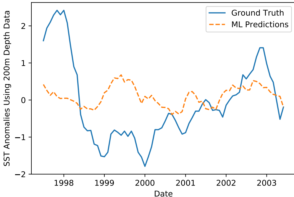
Predicted and True Ocean Temperature Anomalies at 6 Month Lead Time. Corr: 0.18
