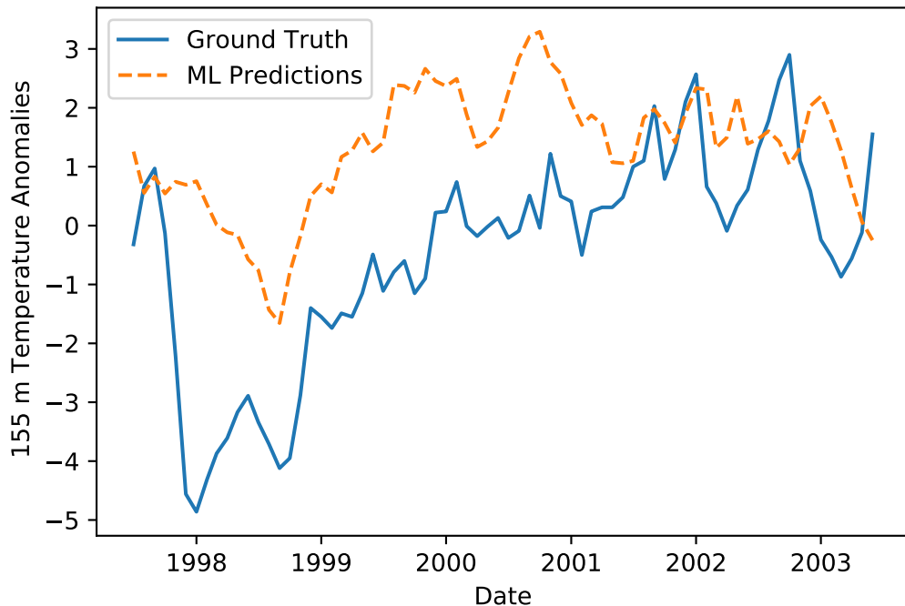
Predicted and True Ocean Temperature Anomalies at 6 Month Lead Time. Corr: 0.61
