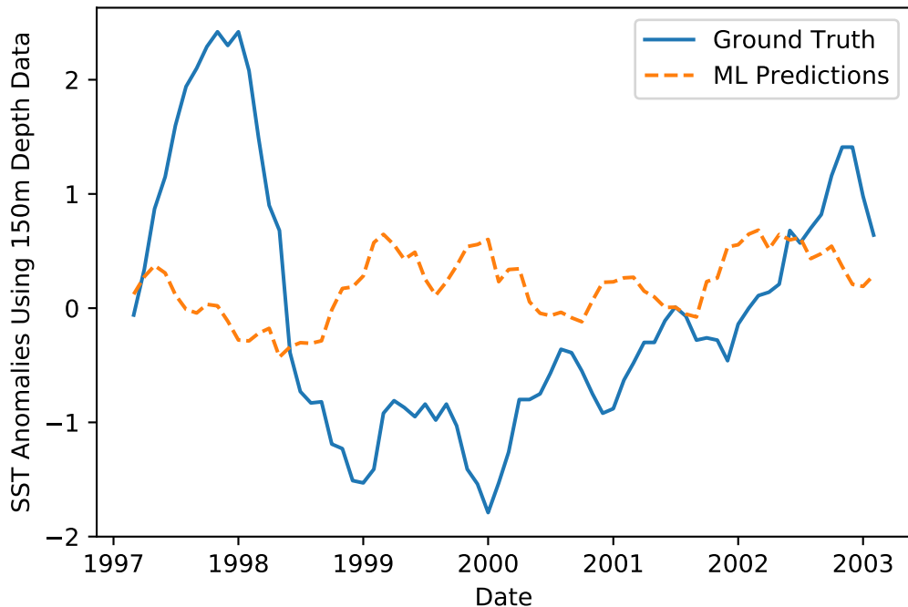
Predicted and True Ocean Temperature Anomalies at 2 Month Lead Time. Corr: -0.25
