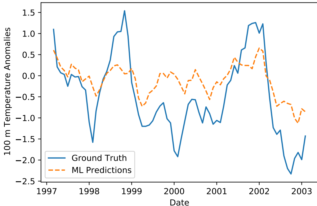
Predicted and True Ocean Temperature Anomalies at 2 Month Lead Time. Corr: 0.79
