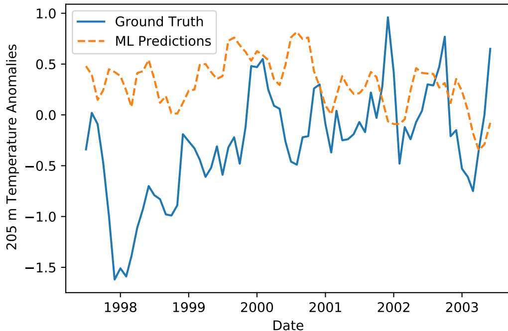
Predicted and True Ocean Temperature Anomalies at 6 Month Lead Time. Corr: -0.00
