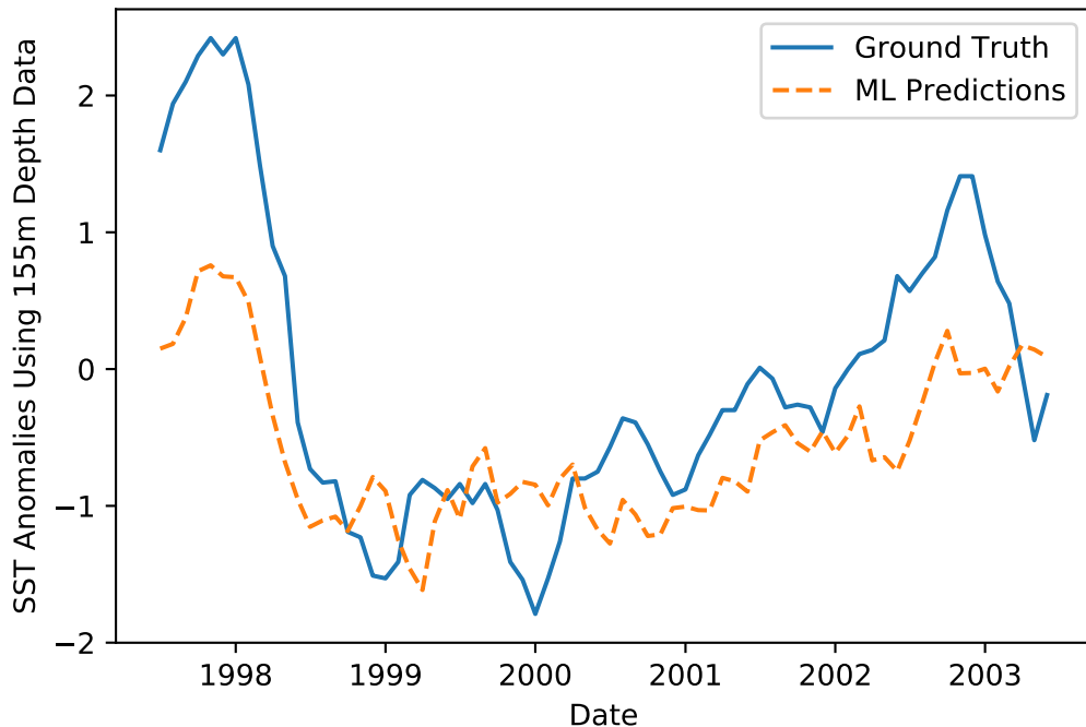
Predicted and True Ocean Temperature Anomalies at 6 Month Lead Time. Corr: 0.85
