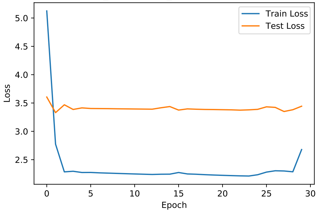
Performance of twolayerCNN_1980-01-01_1995-12-31 Neural Network During Training
