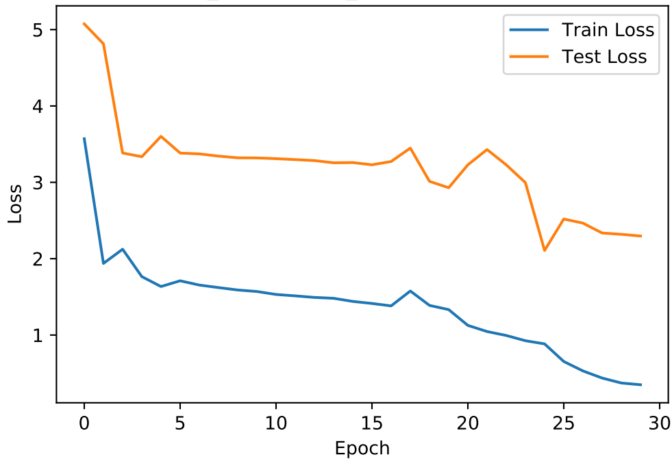
Performance of twolayerCNN_1980-01-01_1995-12-31 Neural Network During Training
