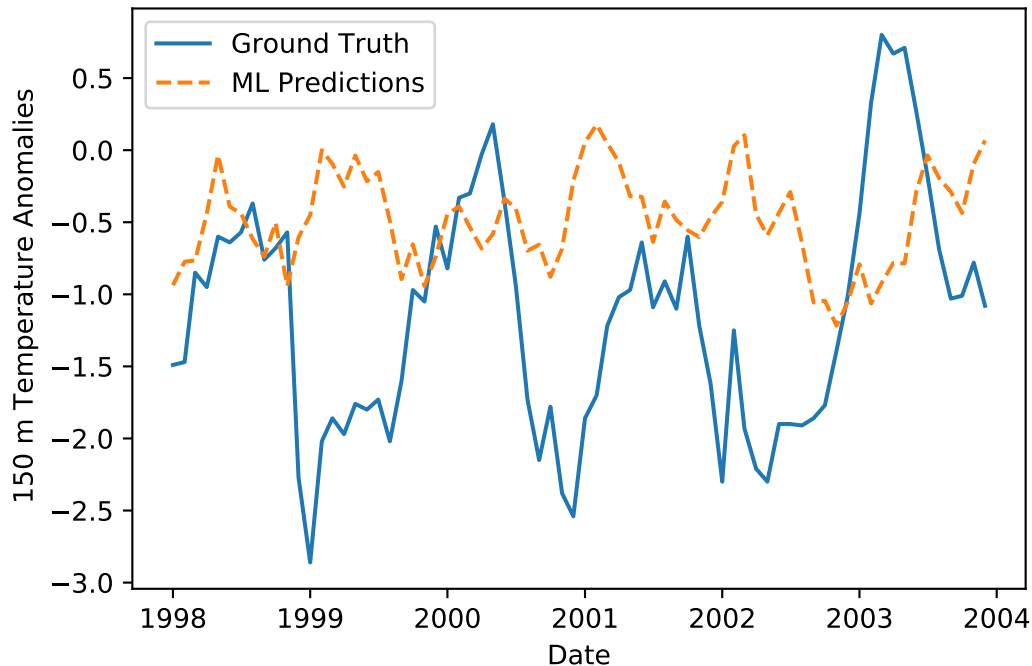
Predicted and True Ocean Temperature Anomalies at 12 Month Lead Time. Corr: -0.19
