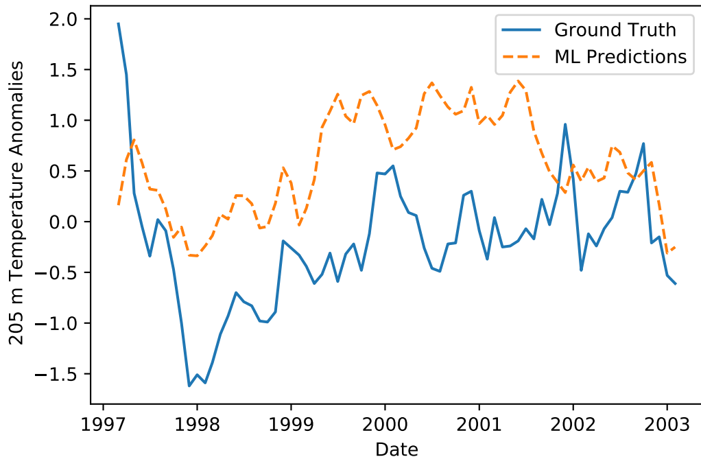
Predicted and True Ocean Temperature Anomalies at 2 Month Lead Time. Corr: 0.38
