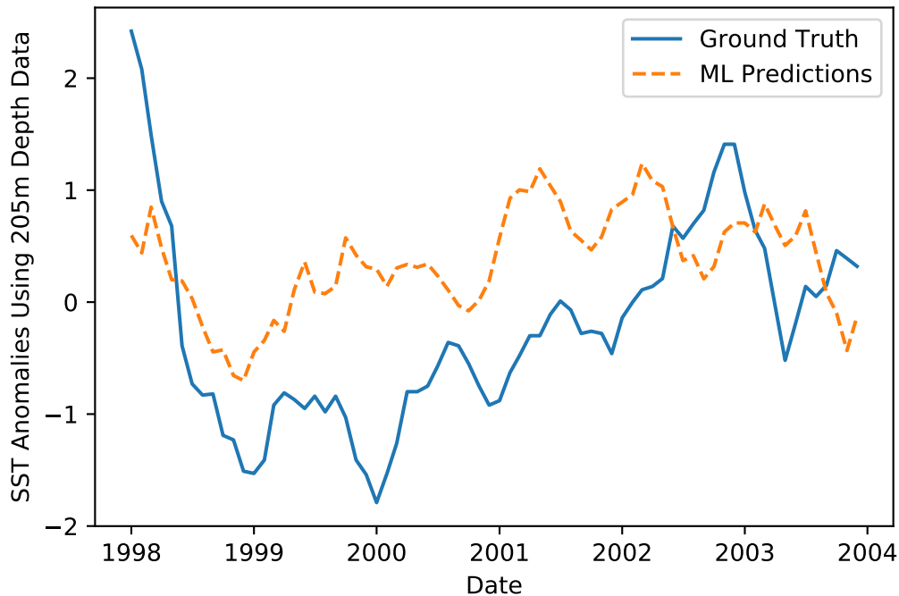
Predicted and True Ocean Temperature Anomalies at 12 Month Lead Time. Corr: 0.41
