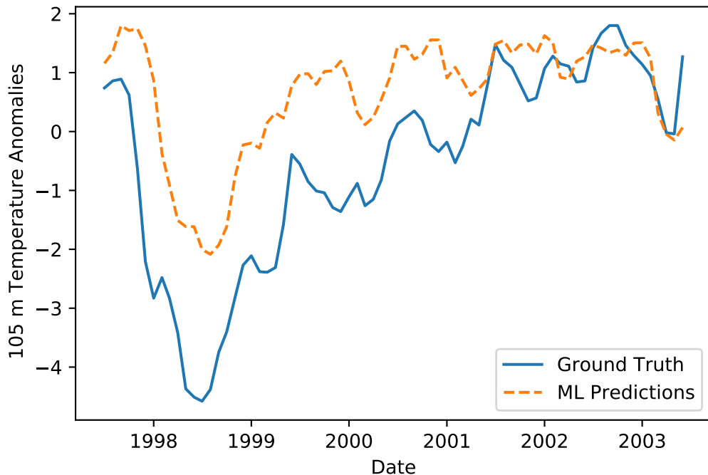
Predicted and True Ocean Temperature Anomalies at 6 Month Lead Time. Corr: 0.83
