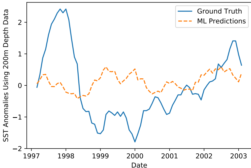
Predicted and True Ocean Temperature Anomalies at 2 Month Lead Time. Corr: -0.12
