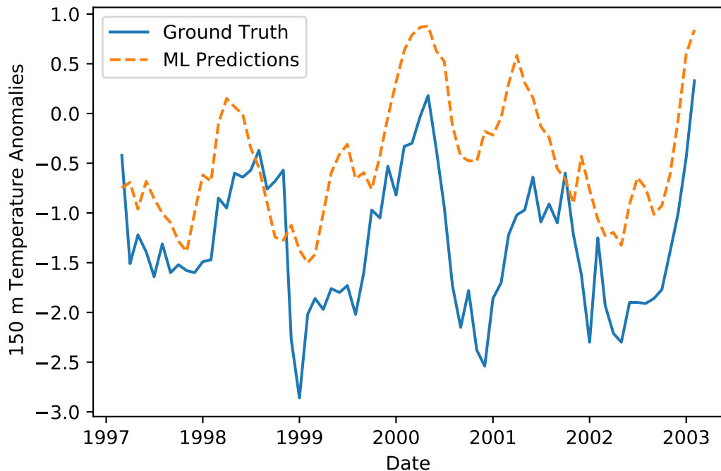
Predicted and True Ocean Temperature Anomalies at 2 Month Lead Time. Corr: 0.62
