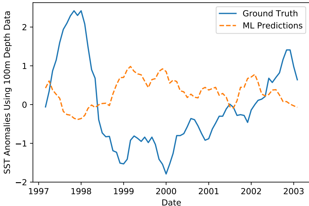
Predicted and True Ocean Temperature Anomalies at 2 Month Lead Time. Corr: -0.76
