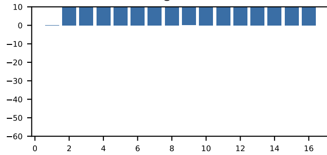
C4 @ 157.05s
