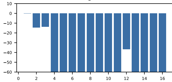
A#3 @ 98.60s
