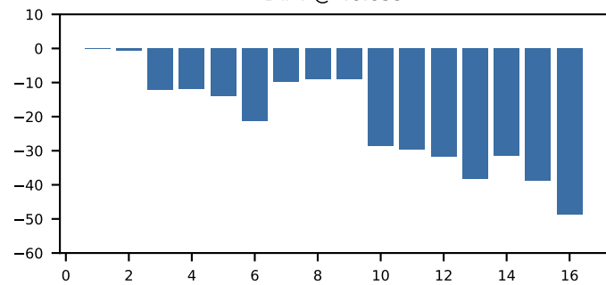
C#4 @ 59.54s
