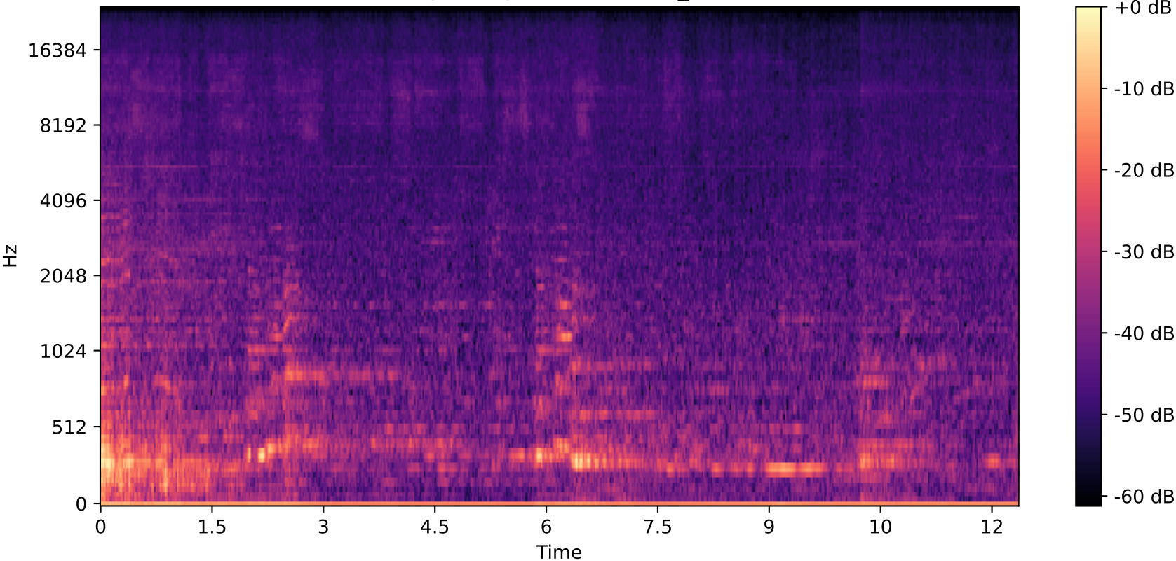
Spectrogram — section_9
