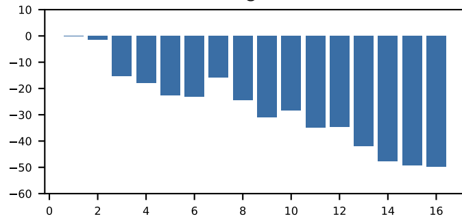
C#4 @ 8.21s
