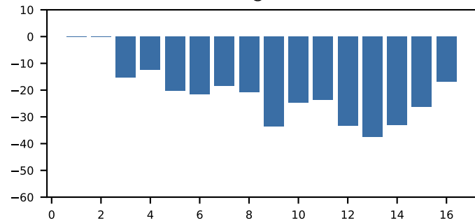
D#4 @ 48.85s
