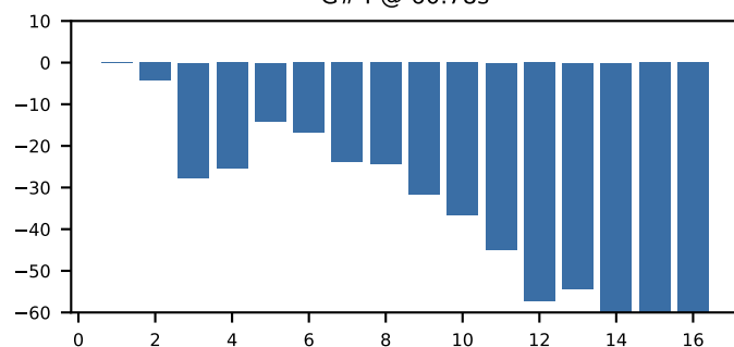
G#4 @ 60.78s
