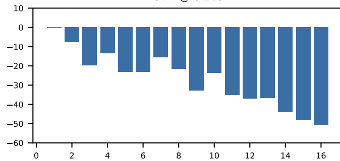
D#4 @ 50.82s
