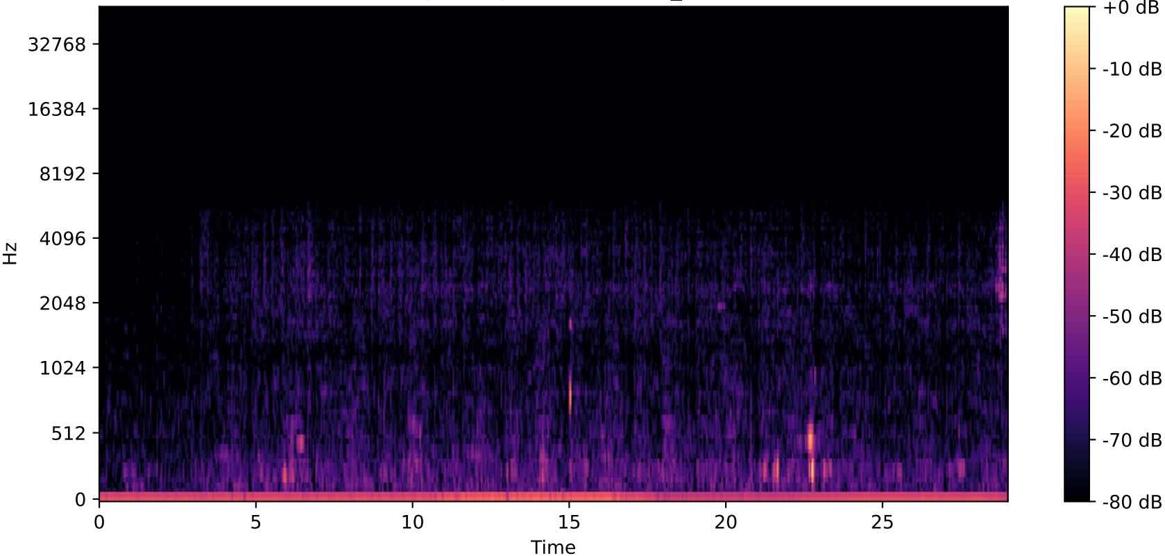
Spectrogram — section_9
