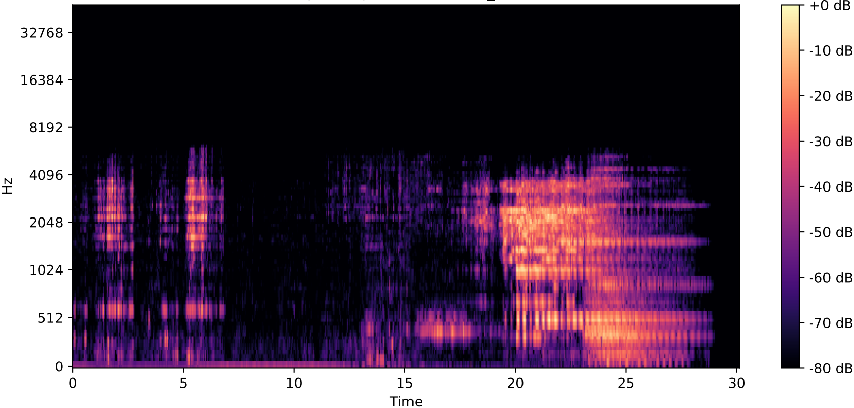
Spectrogram — section_10
