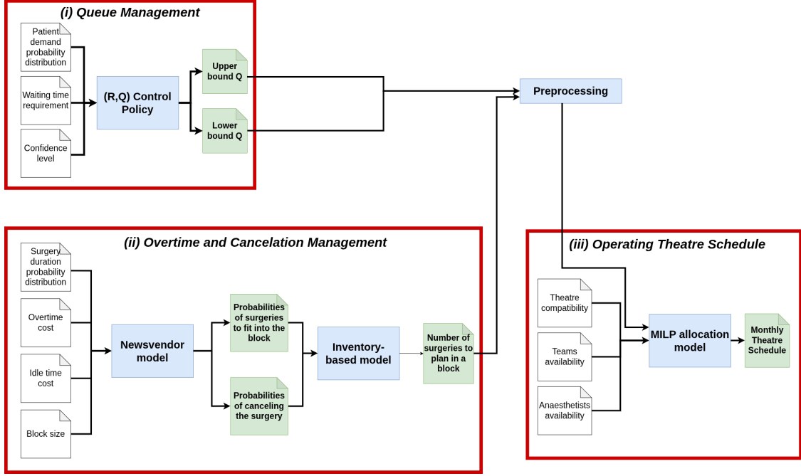
Figure 3: Proposed framework.
