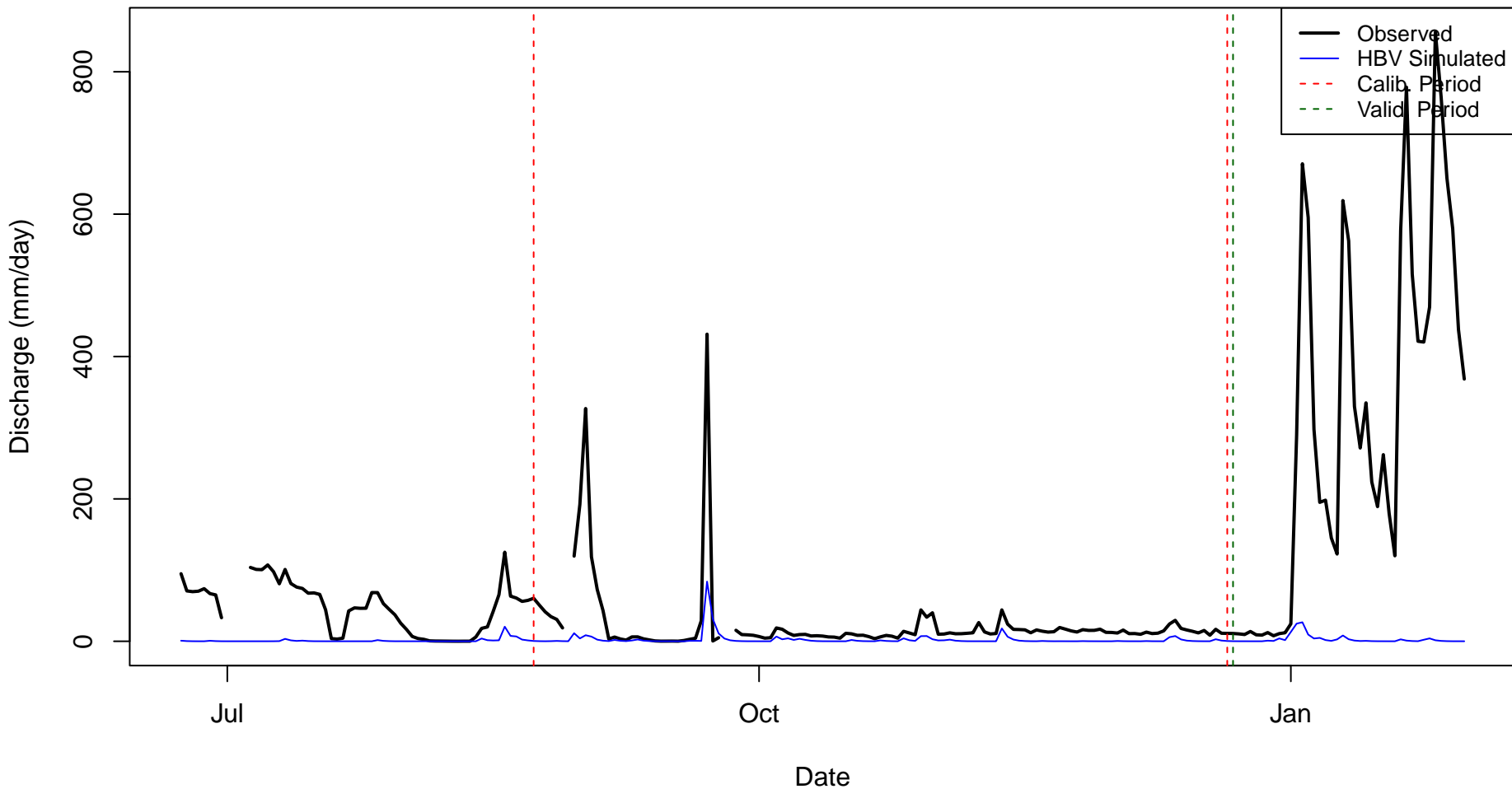
Observed vs Simulated Discharge (HBV Model)
