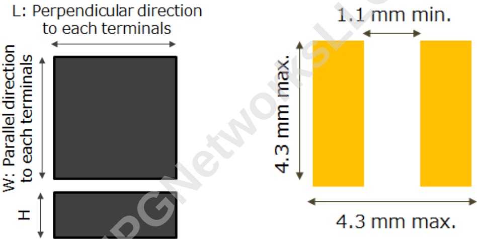
Figure 32 — Reference Drawing and Recommended Land Pattern
