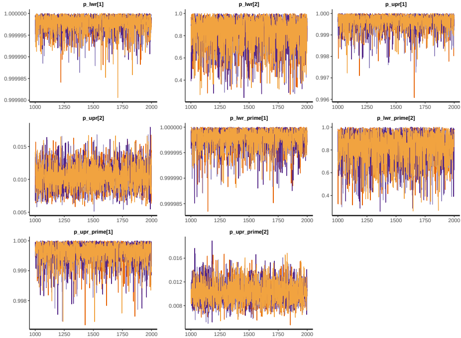
Figure 3: MCMC parameter traceplots applied to A. bipustulatus ([1]; N = 701 ) and A. nevadensis ([2]; N = 2 ) for CYTB across 1000 post-warmup iterations.
