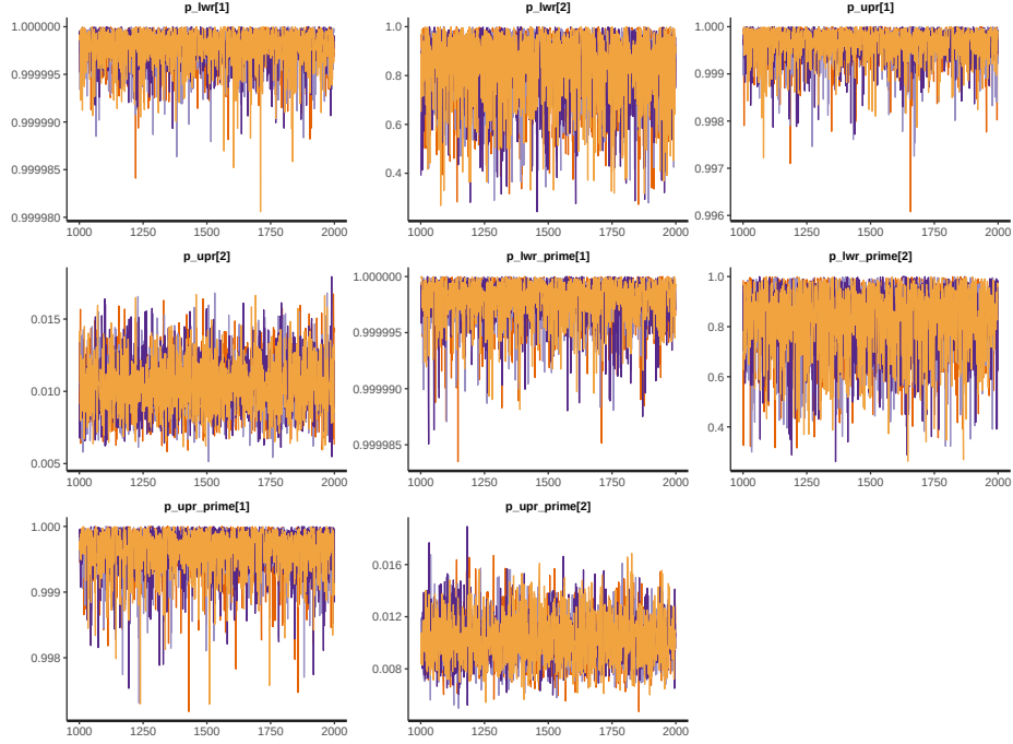
Figure 4: MCMC parameter traceplots applied to A. bipustulatus ([1]; N = 701 ) and A. nevadensis ([2]; N = 2 ) for CYTB across 1000 post-warmup iterations.
