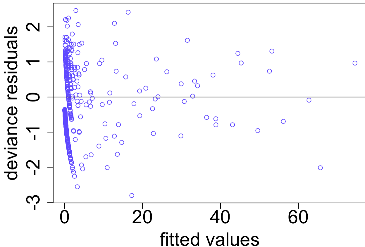
Figure 6: Conventional residual plots for Poisson GLMM
