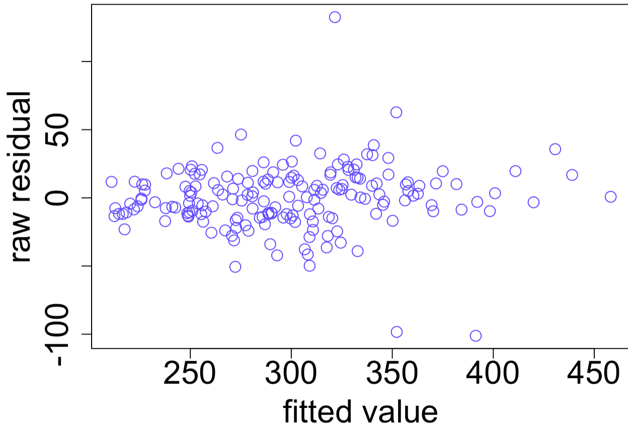
Figure 1: A typical LMM residual pattern
