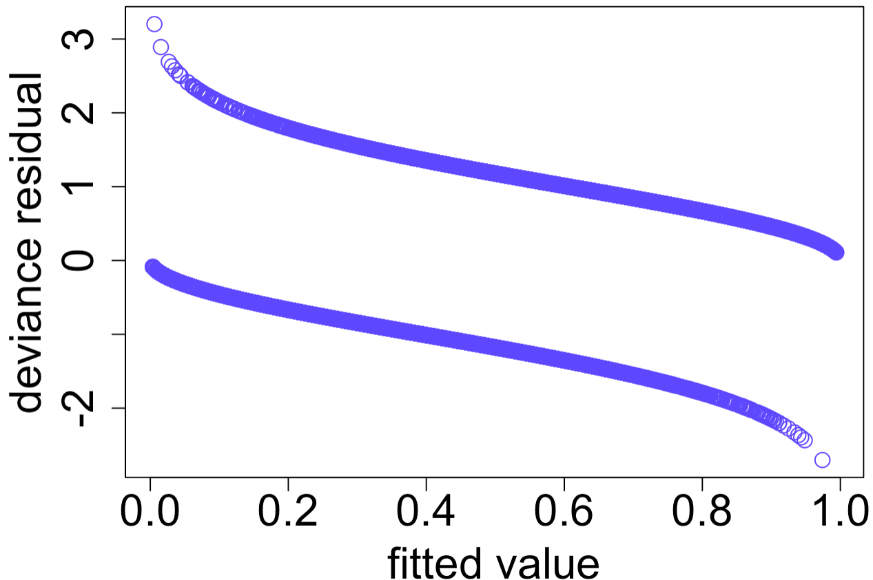
Figure 2: Residual plot for a binomial-distributed variable
