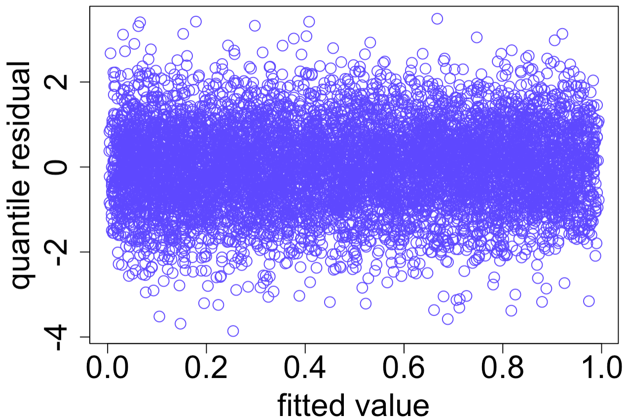
Figure 12: glmmTMB quantile residuals
