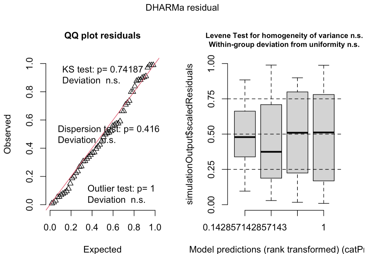
Figure 11: Unconditional simulation of a glmer object
