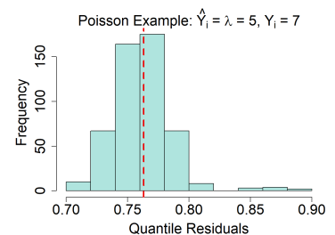
Figure 4: Quantile Residuals (500 simulations of 500 obs each)
