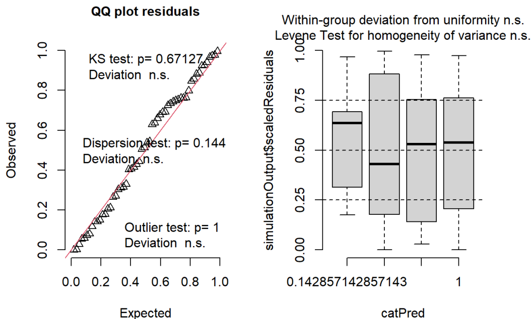
Figure 10: Unconditional simulations of a glmmTMB object
