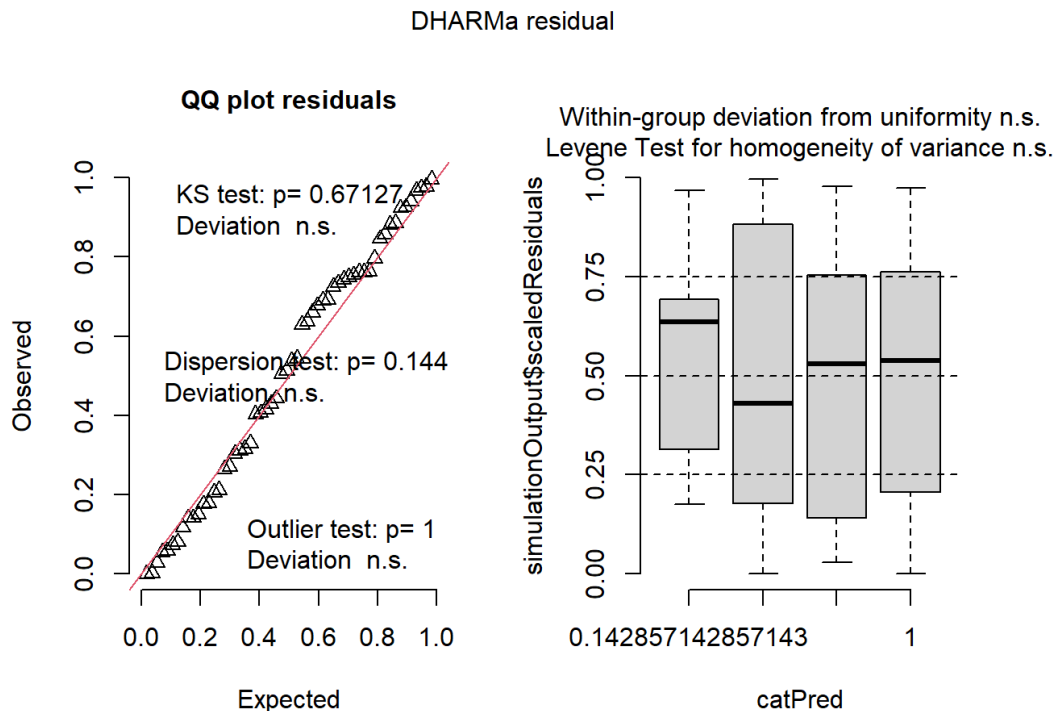
Figure 11: Conditional simulation of a glmer object
