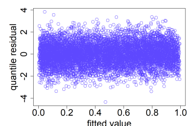
Figure 13: glmmTMB quantile residuals
