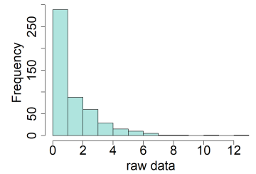
Figure 5: Histogram of the Poisson variable simulated by DHARMA
