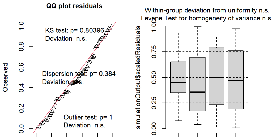
DHARMA residual
