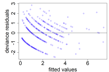
Figure 6: Conventional residual plots for Poisson GLMM
