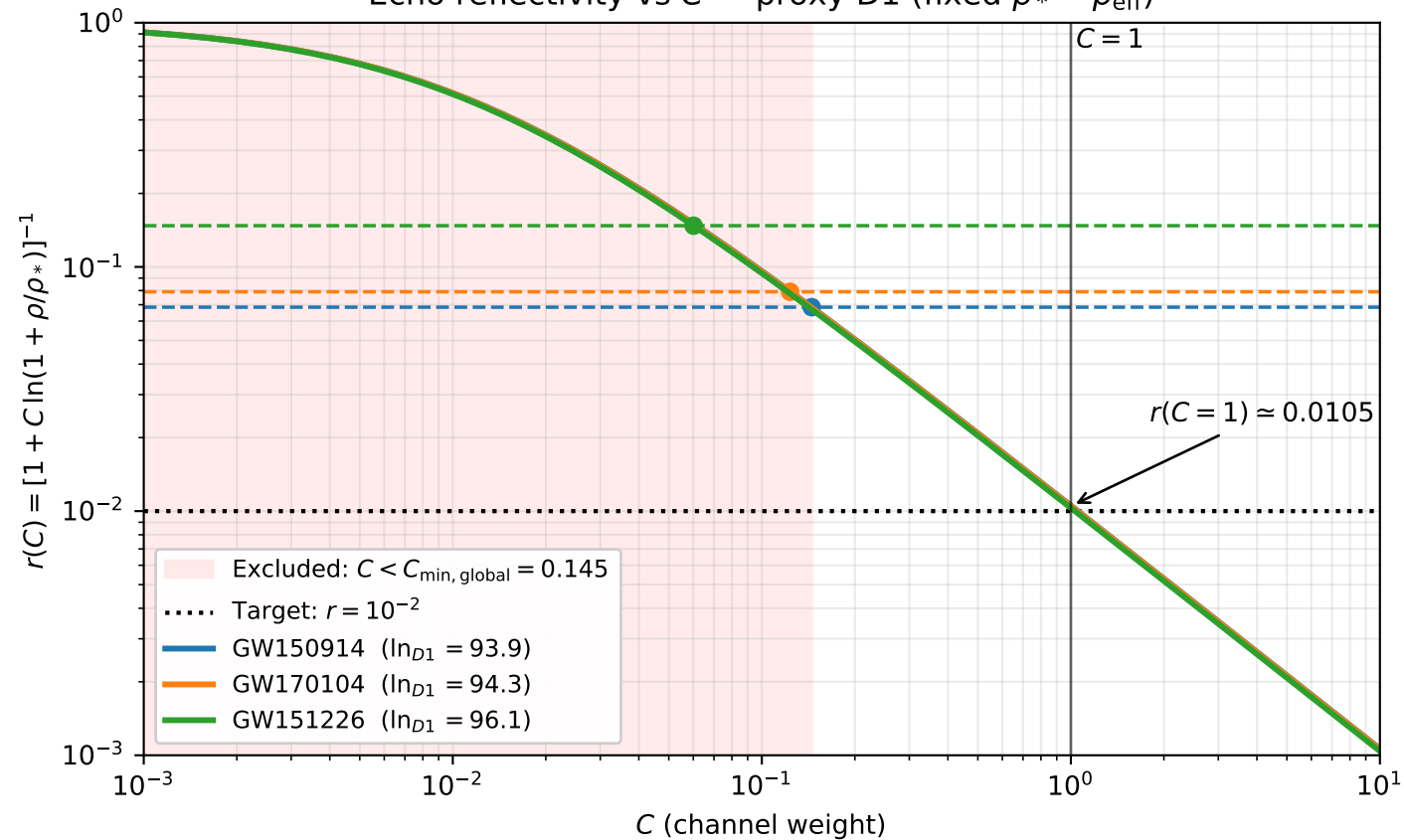
Echo reflectivity vs C — proxy D1 (fixed \rho_* = \rho_{\text{eff}} )
