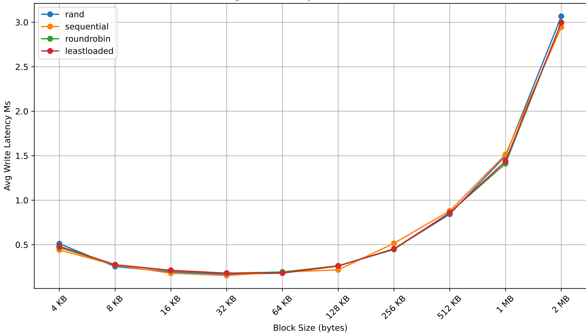
Avg Write Latency Ms vs Block Size
