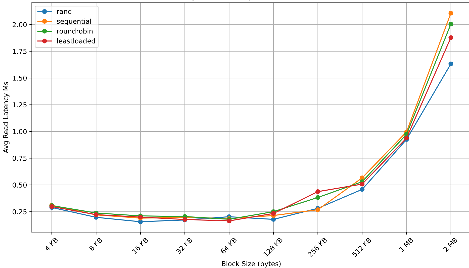
Avg Read Latency Ms vs Block Size
