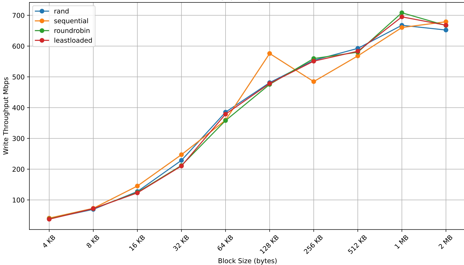
Write Throughput Mbps vs Block Size
