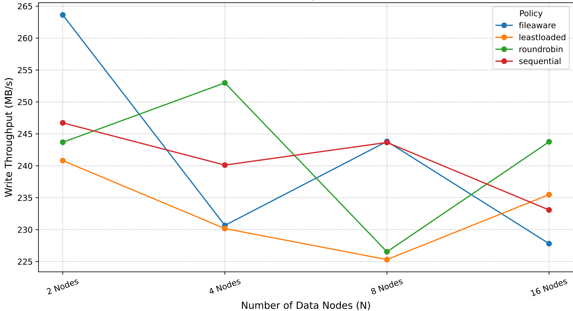
Write Throughput (MB/s) vs. Data Node Count (Workload: Uniform Large, Block Size: 32 KB)
