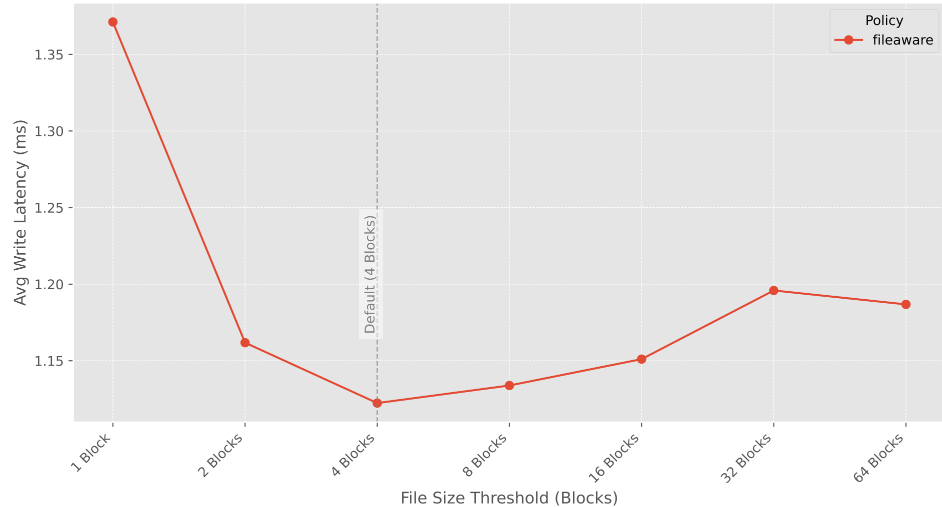
File Aware Policy Tuning: Avg Write Latency (ms) (Workload: Uniform Large, Block Size: 4 KB)
