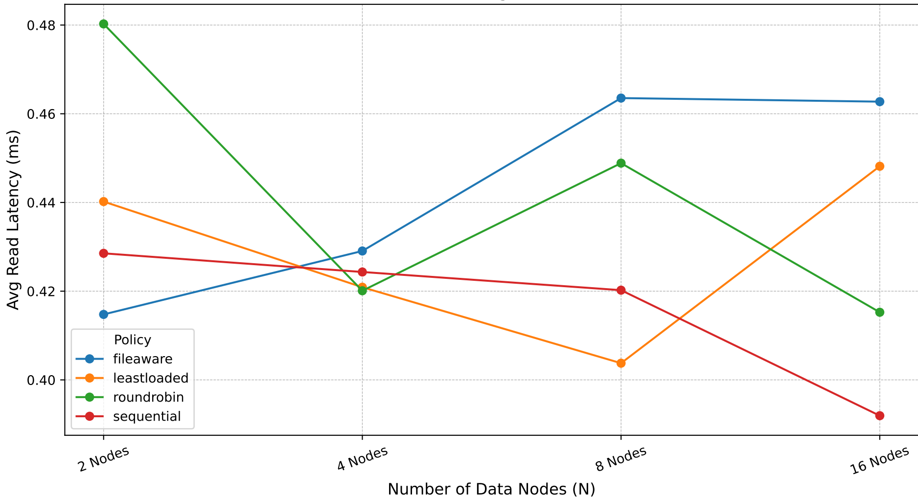
Avg Read Latency (ms) vs. Data Node Count (Workload: Uniform Large, Block Size: 32 KB)
