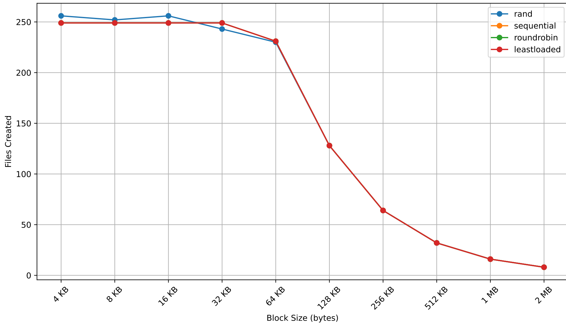
Files Created vs Block Size
