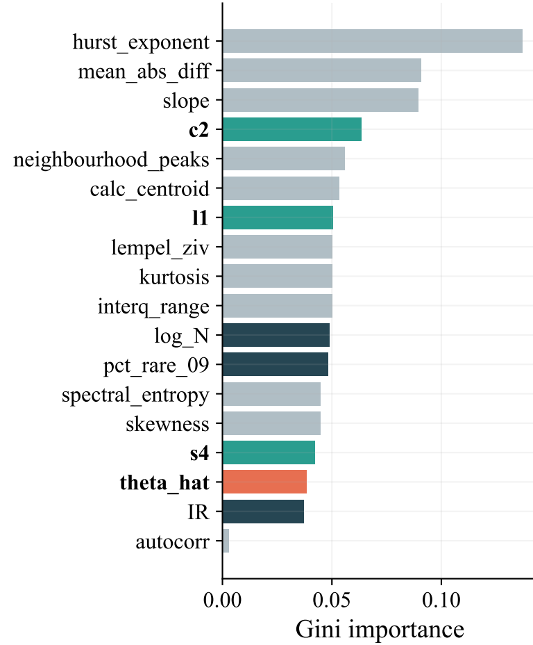
(a) best learner
