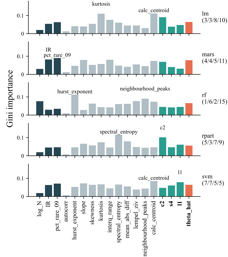
(c) best resampling family, per base learner
