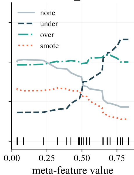
theta_hat
