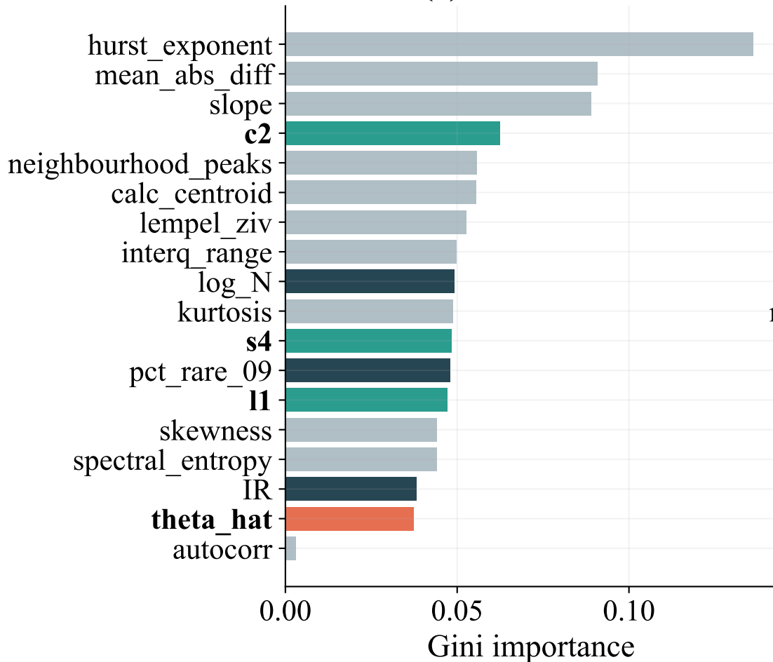
(a) best learner
