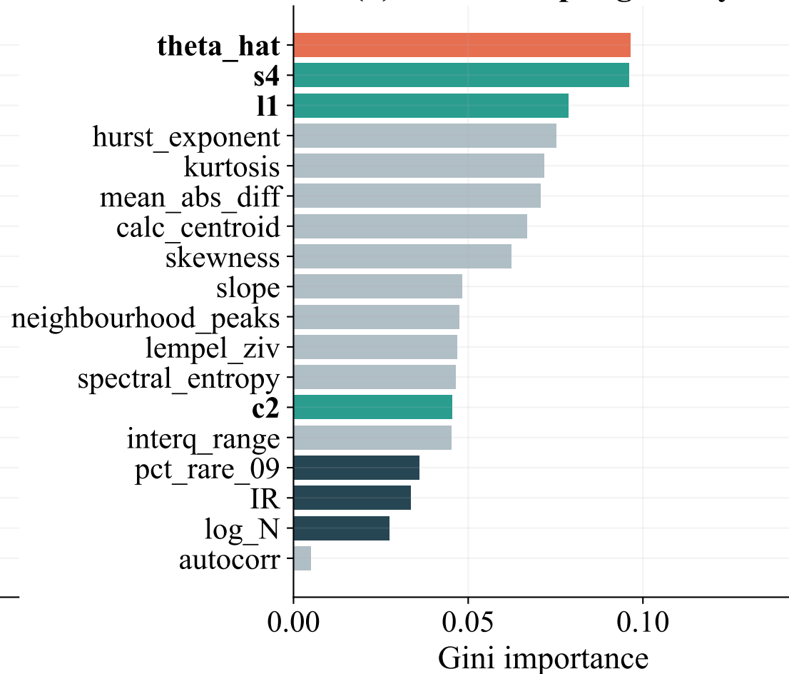
(b) best resampling family
