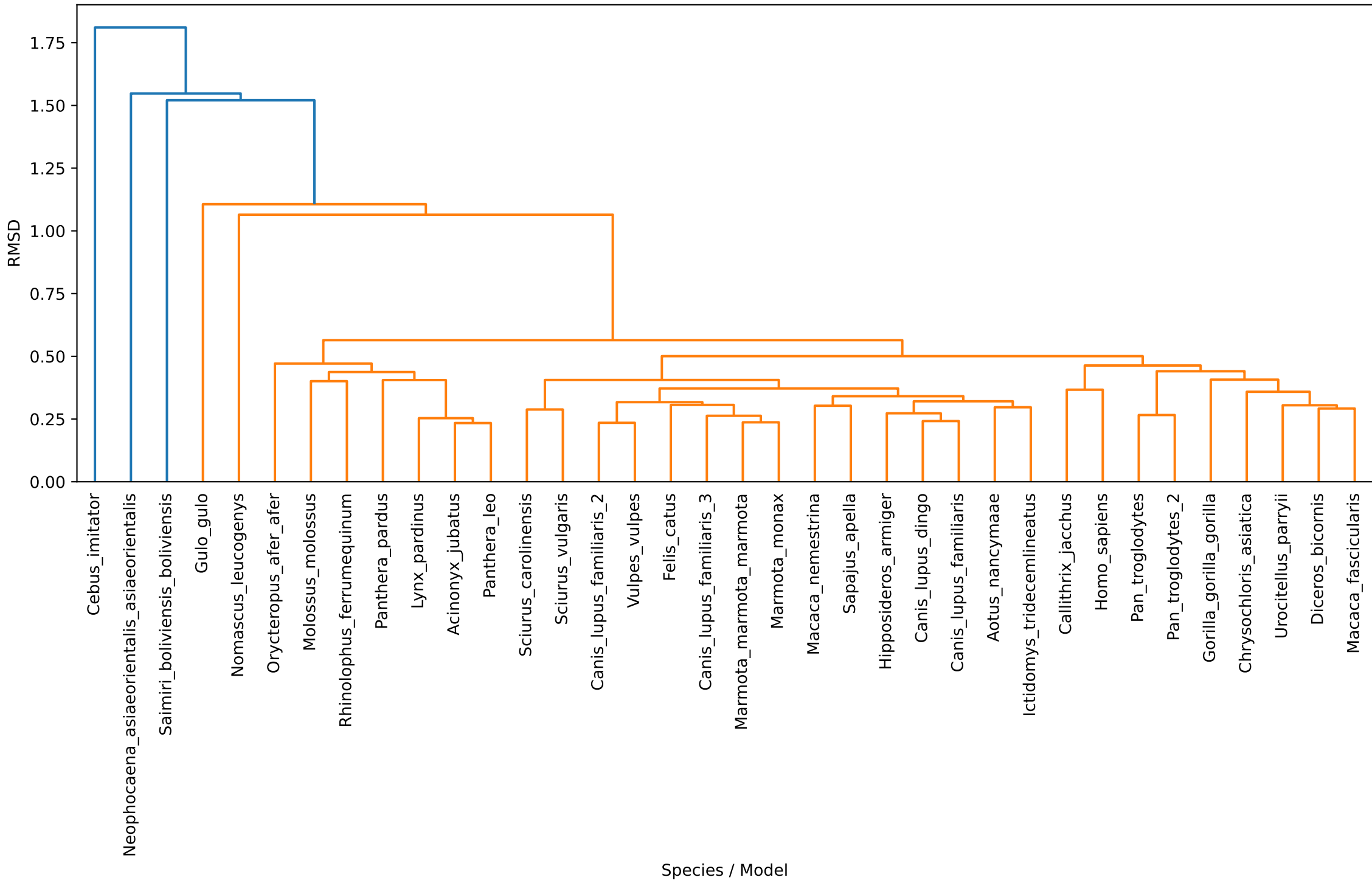
Hierarchical Clustering of Models based on RMSD (Average Linkage)
