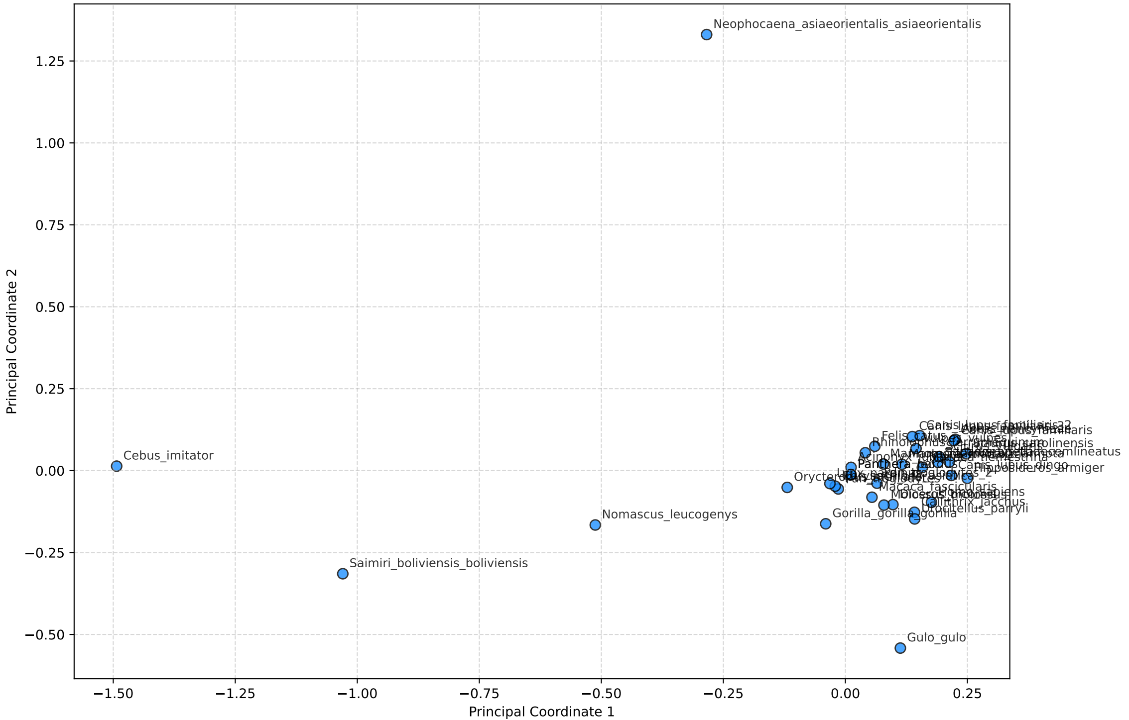
Principal Coordinate Analysis (PCoA / PCA) of RMSD Matrix
