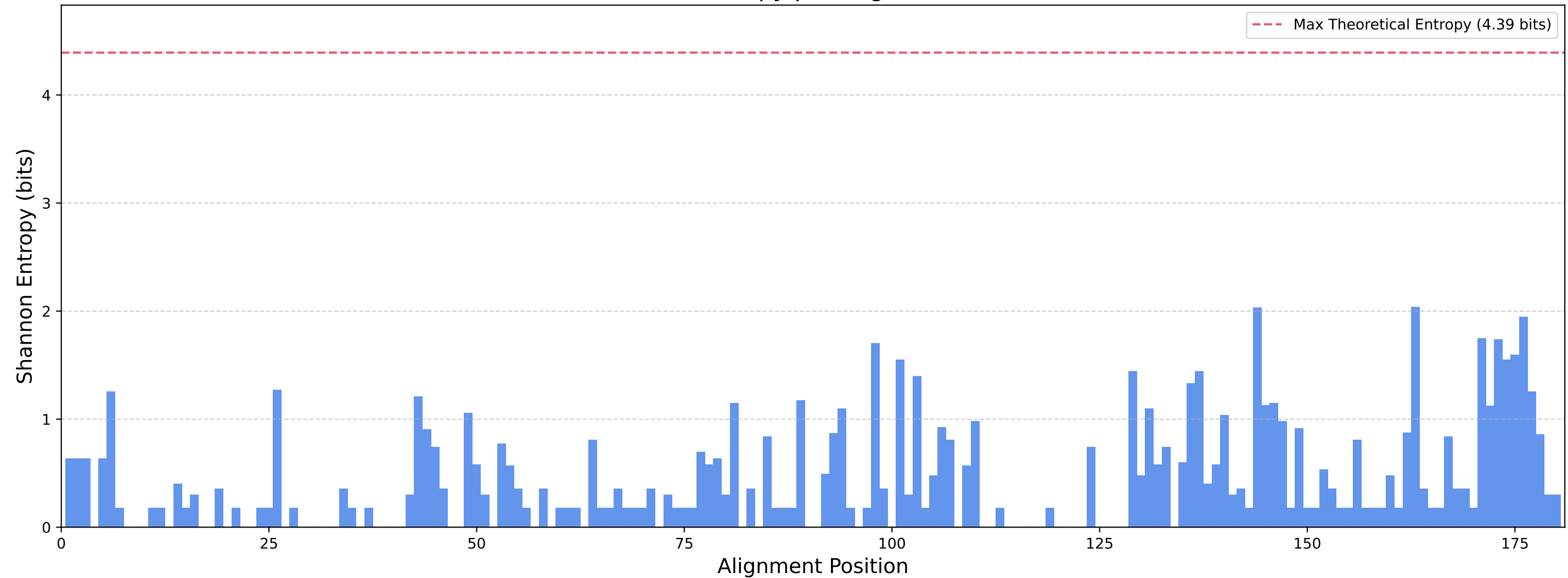
Shannon's Entropy per Alignment Position
