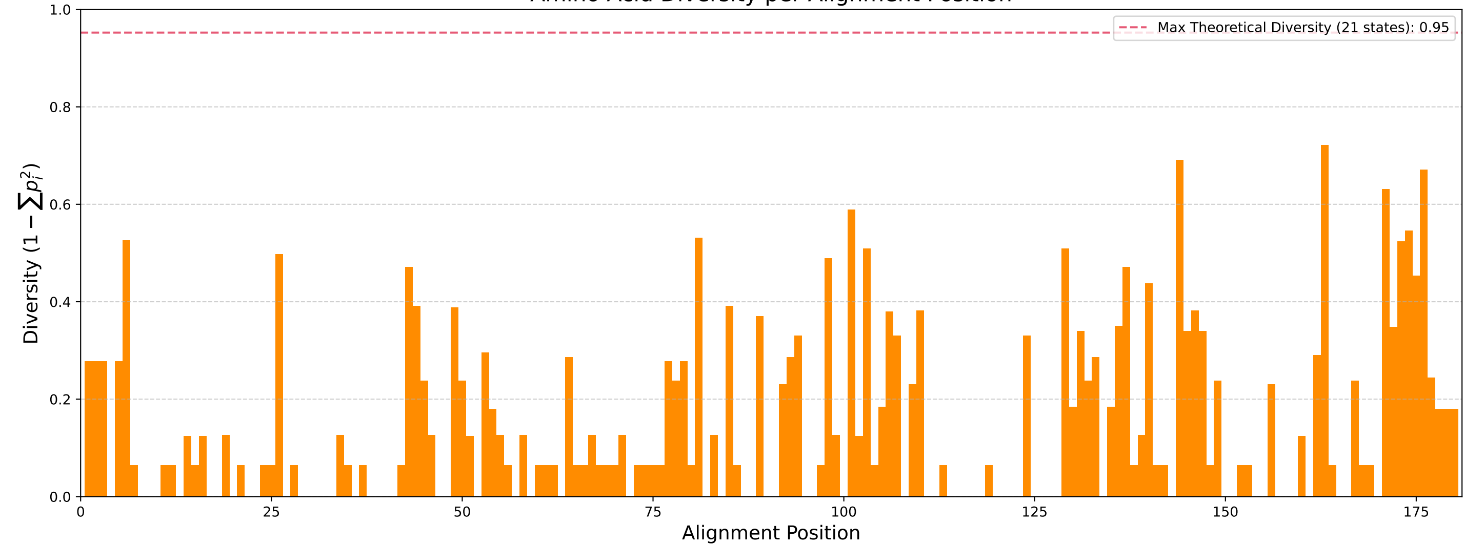
Amino Acid Diversity per Alignment Position
