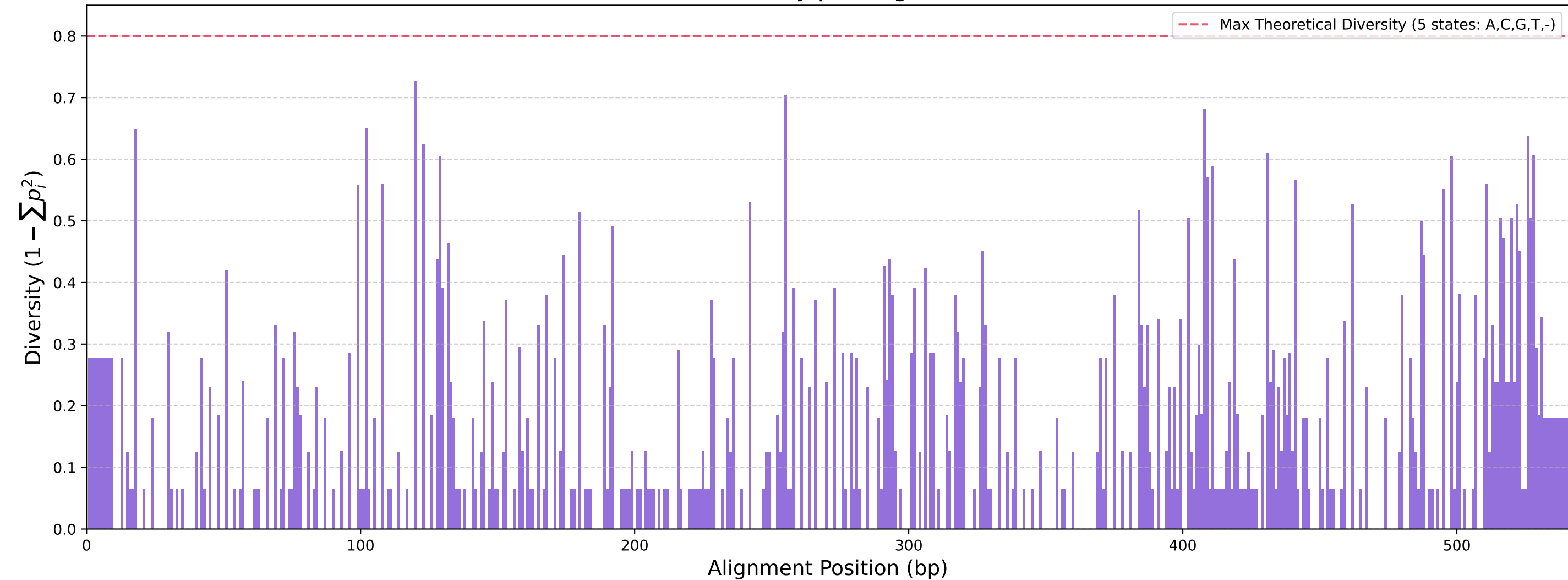
Nucleotide Diversity per Alignment Position
