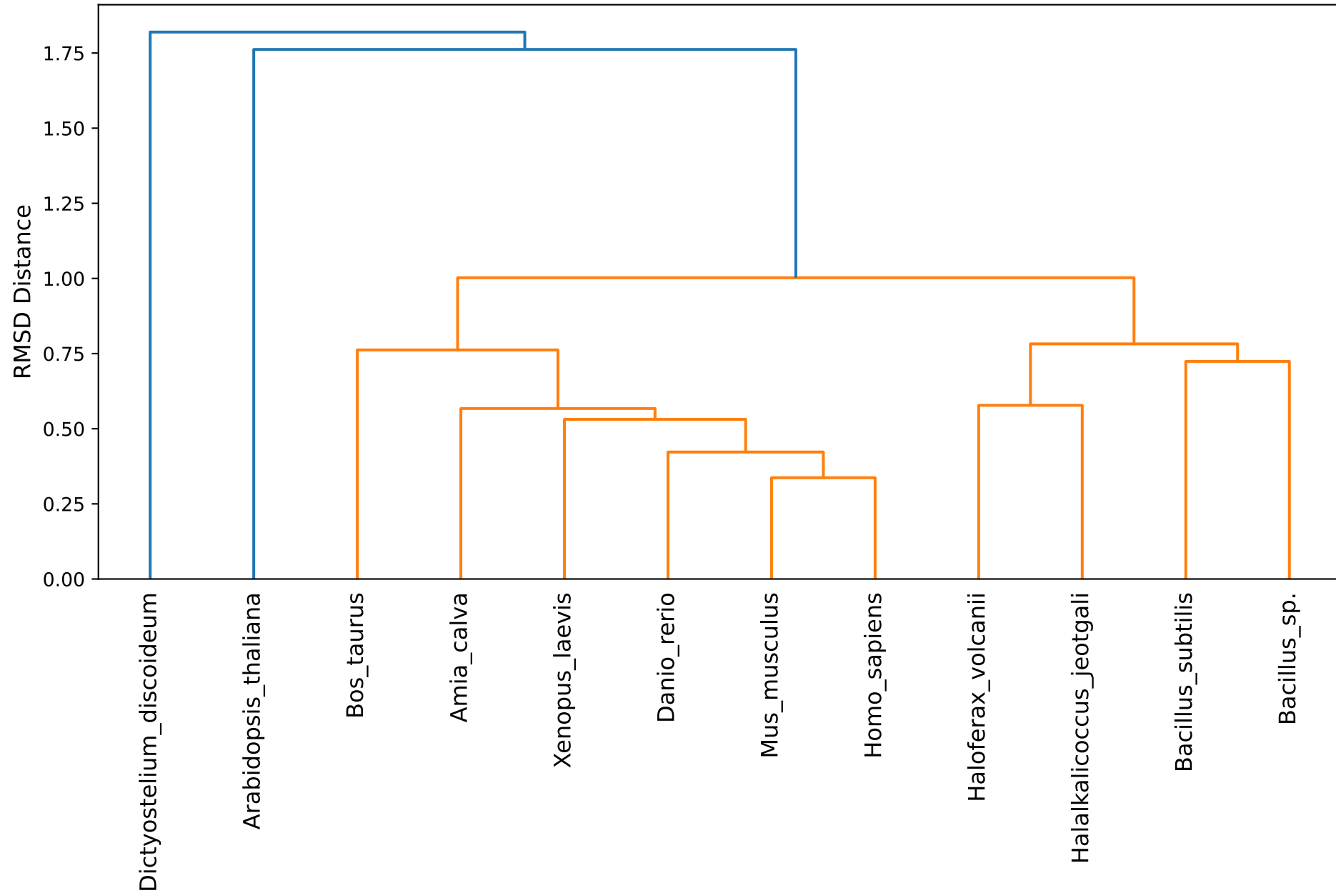
Hierarchical Clustering based on RMSD (12 Models)
