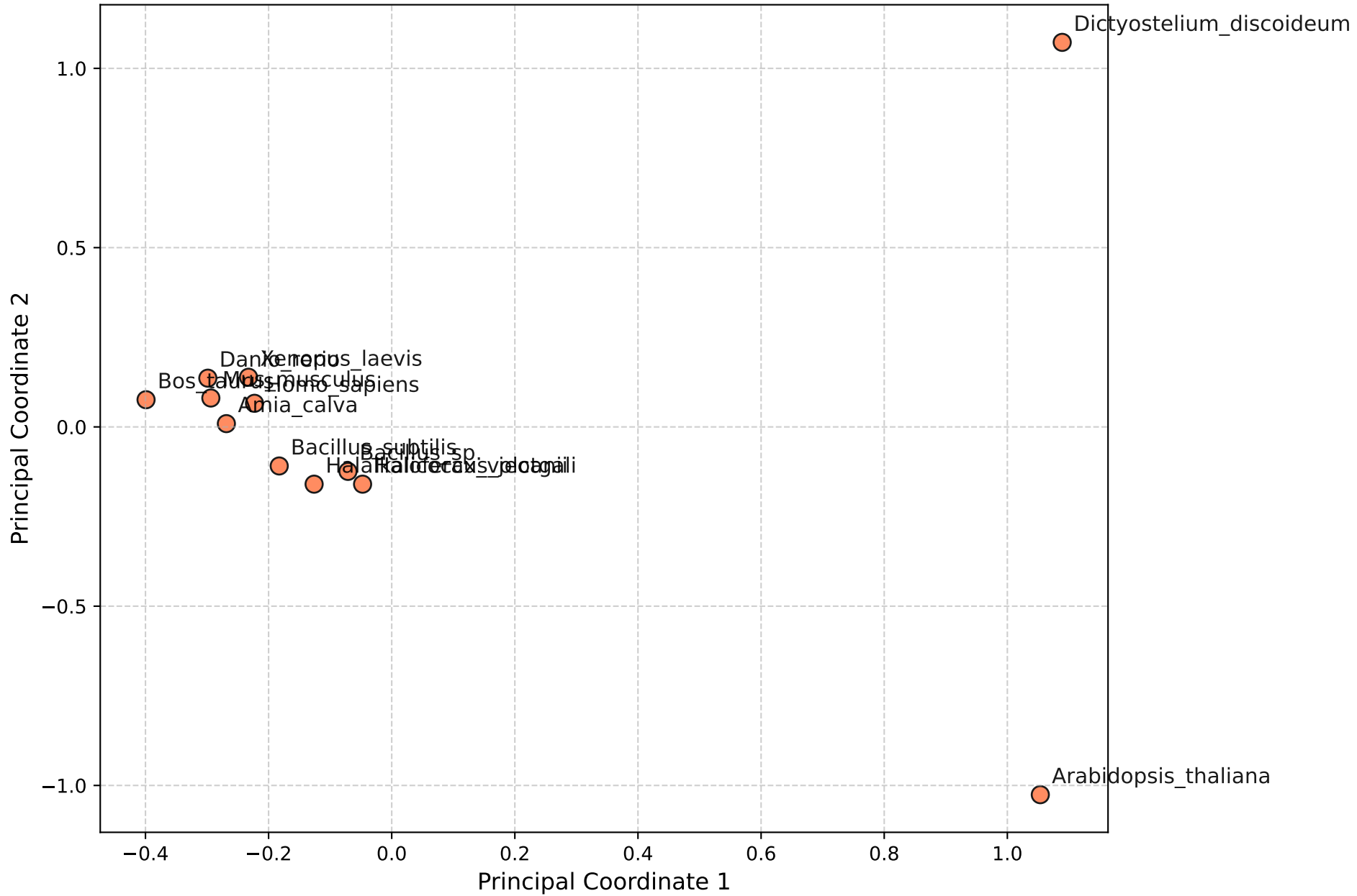
Principal Coordinate Analysis (PCoA) of RMSD Matrix
