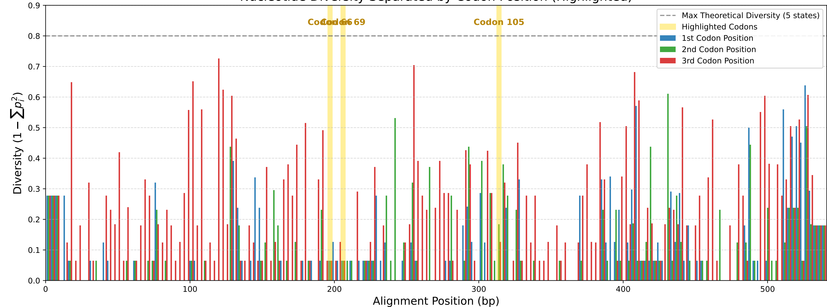
Nucleotide Diversity Separated by Codon Position (Highlighted)
