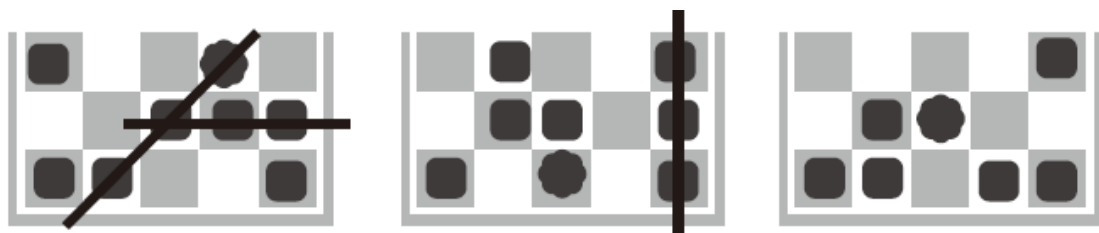
the third board is invalid, no formation exists
