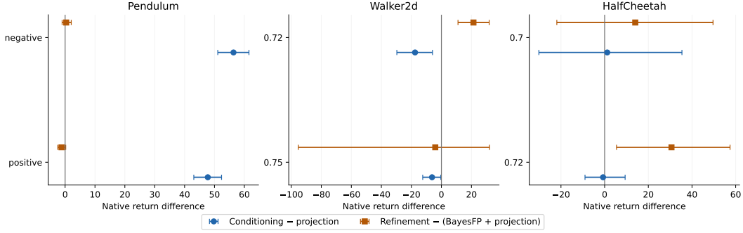
Figure 1: Target utility and finite-sampler performance are separate comparisons. The horizontal axes use each task’s native return units. Q–P intervals are 95% for Pendulum and 99.375% for MuJoCo; R–(B+P) intervals are 98.75% and 99.375%, respectively. They follow the separate predeclared comparison families described in the text.
