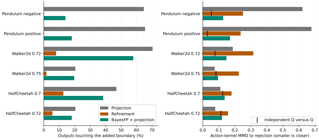
Figure 2: Boundary concentration and finite-sample action-kernel discrepancy. The independent Q-versus-Q marker indicates sampling noise, not a formal threshold. Kernel RMS bandwidth is .1 for normalized Pendulum actions and .2 for MuJoCo actions. MMD values therefore should not be compared directly across tasks. The added safety boundary is distinct from pre-existing physical action saturation.
