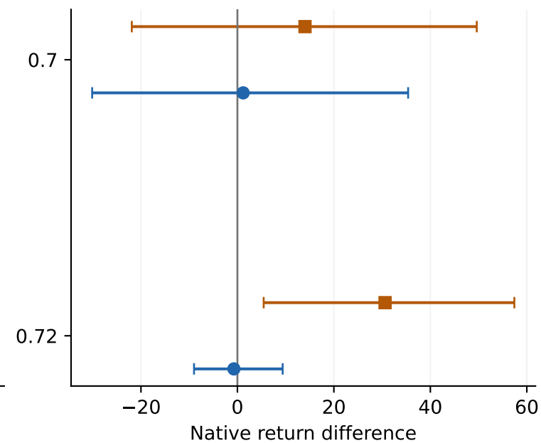
HalfCheetah
