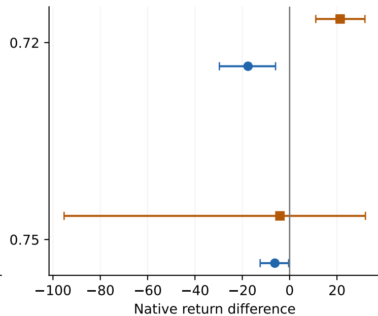
Walker2d
