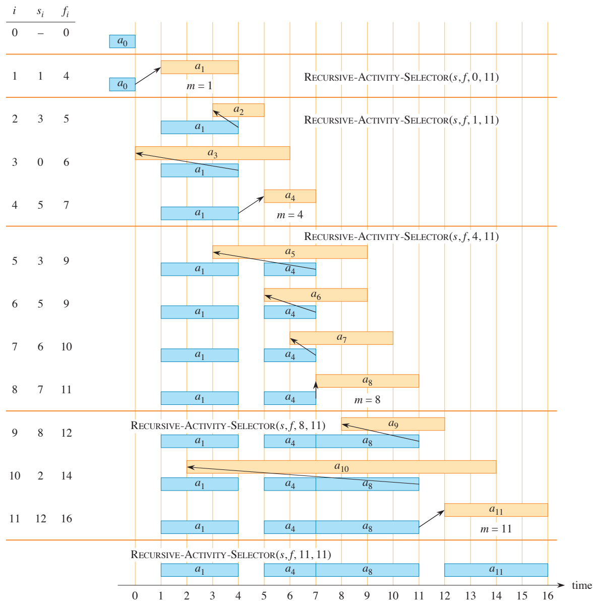
Figure 15.2 The operation of \text{RECURSIVE-ACTIVITY-SELECTOR} on the 11 activities from Figure 15.1. Activities considered in each recursive call appear between horizontal lines. The fictitious activity a_0 finishes at time 0, and the initial call \text{RECURSIVE-ACTIVITY-SELECTOR}(s, f, 0, 11) , selects activity a_1 . In each recursive call, the activities that have already been selected are blue, and the activity shown in tan is being considered. If the starting time of an activity occurs before the finish time of the most recently added activity (the arrow between them points left), it is rejected. Otherwise (the arrow points directly up or to the right), it is selected. The last recursive call, \text{RECURSIVE-ACTIVITY-SELECTOR}(s, f, 11, 11) , returns \emptyset . The resulting set of selected activities is \{a_1, a_4, a_8, a_{11}\} .
