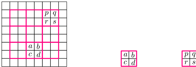
Figure 11: ad - bc = \pm 1, ps - qr = \pm 1 , Example 1.23
