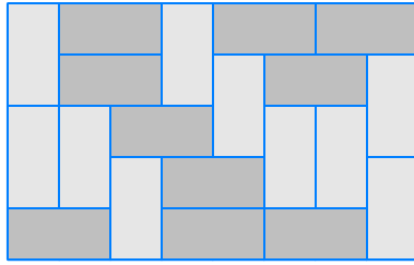
Figure 7: India BMath 2006 (a tiling of a 5 \times 8 rectangle with non-overlapping dominoes), Example 1.10
