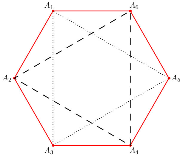
Figure 1: India IOQM 2023 P16, Exercise 1.2
