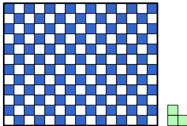
Figure 6: Tiling a 12 \times 15 chessboard using trominos.
