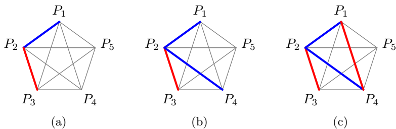
Figure 2: SMMC 2017 A1, Exercise 1.3, First two colored segments share a common vertex
