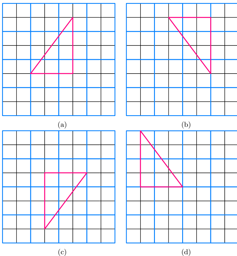
Figure 10: India RMO 2017b P1 — Several configurations of triangles with side lengths (3, 4, 5) , Example 1.21
