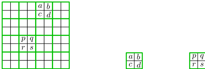
Figure 12: ad - bc = \pm 1, ps - qr = \pm 1 , Example 1.23
