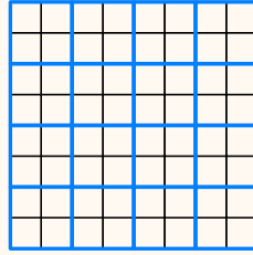
Figure 13: Moscow MO 2015 Grade 11 Day 1 P5, Example 1.23
