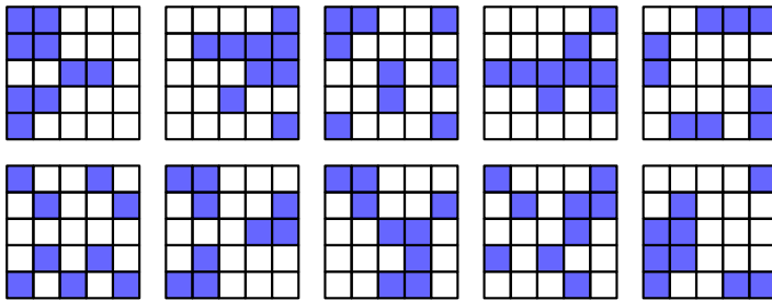
Figure 14: USAMO 2000 P4, Exercise 1.25
