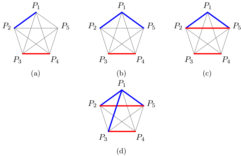
Figure 3: SMMC 2017 A1, Exercise 1.3, First two colored segments share no common vertex
