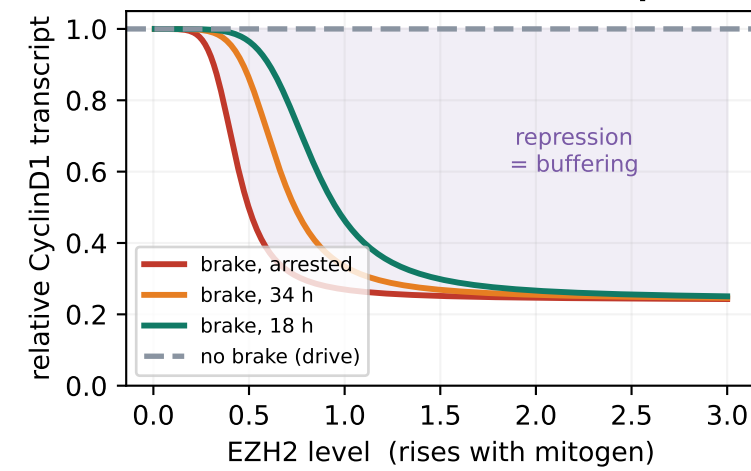
(C) Throttle: more EZH2 → more mark → less transcript
