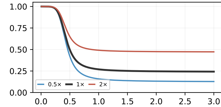
f0_mk — leak floor
