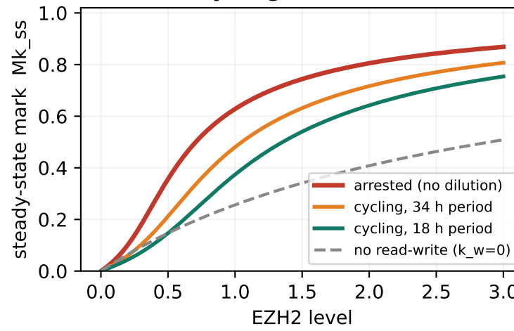
(B) Writing vs erasing: faster cycling dilutes the mark
