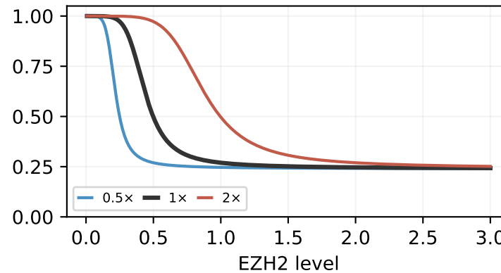
del_mk — demethylation / turnover
