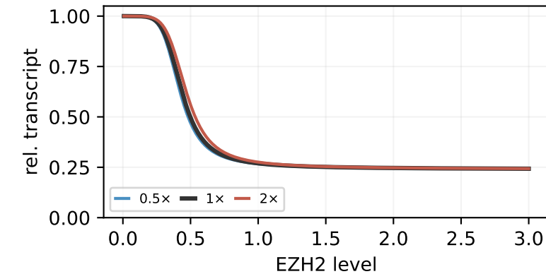
g_mk — transcription eviction
