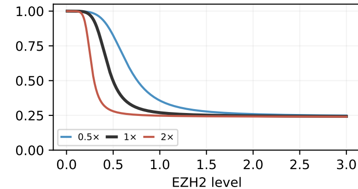
k_w_mk — read-write autocatalysis
