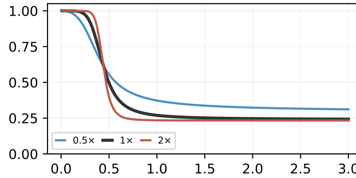
n_mk — switch steepness
