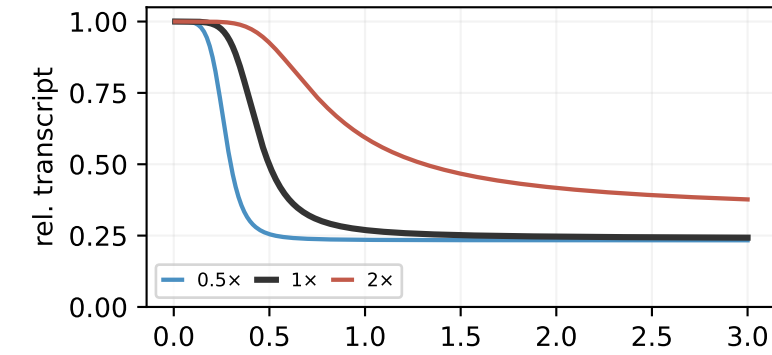
K_mk — mark→repression midpoint
