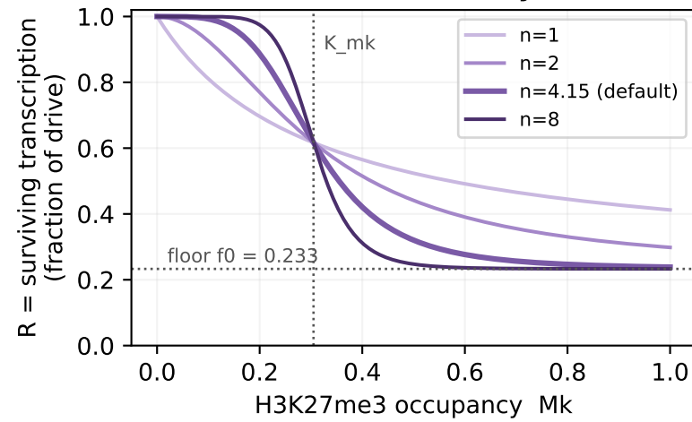
(A) Readout: the mark throttles, never silences (leaky Hill)
