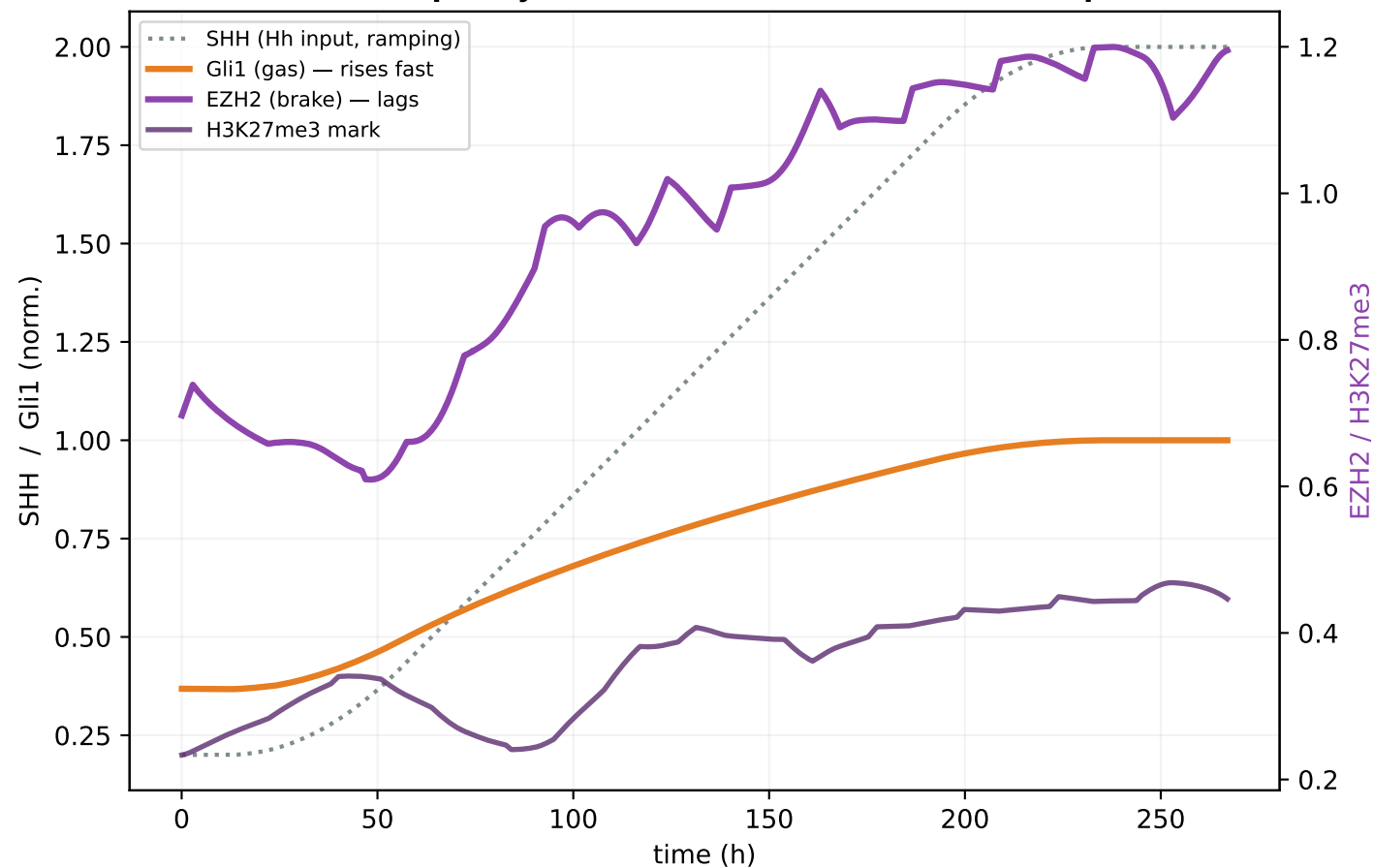
(A) Gradually rising Hh: the gas leads, the brake lags Gli1 tracks Hh quickly; slow \text{EZH2} \rightarrow \text{H3K27me3} catches up behind
