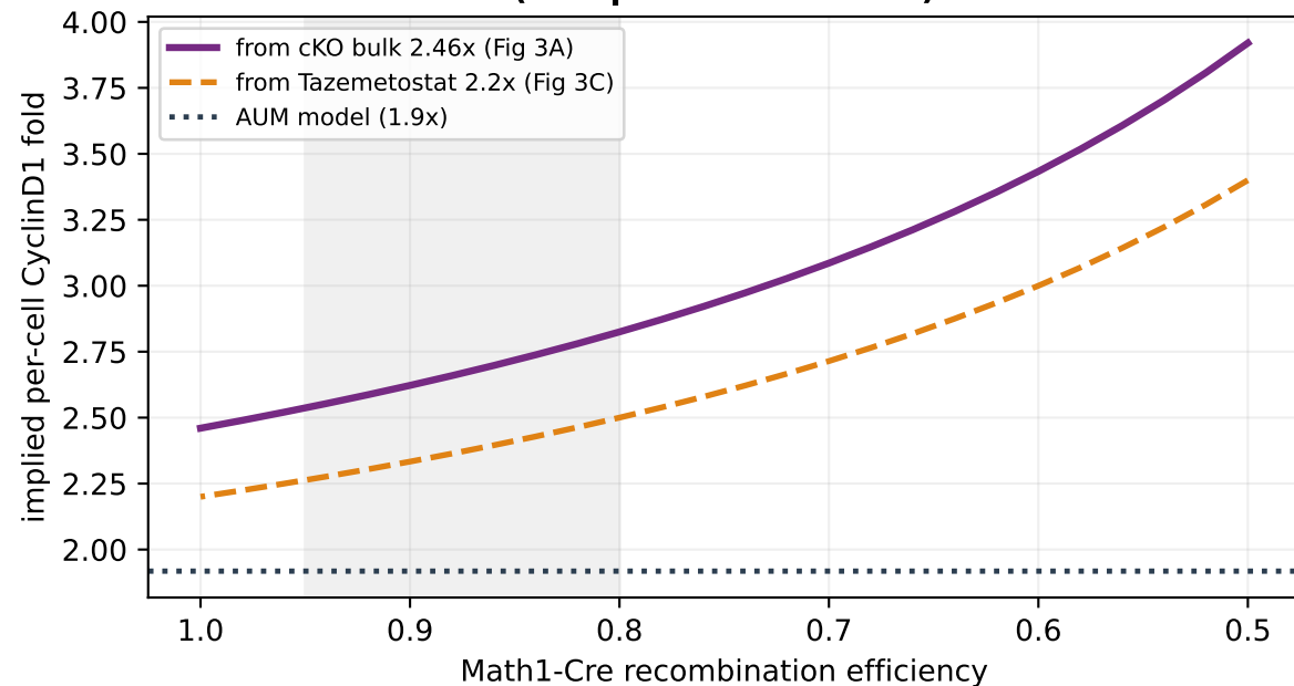
(a) The bulk cKO fold UNDER-estimates per-cell de-repression (escaper cells dilute it)
