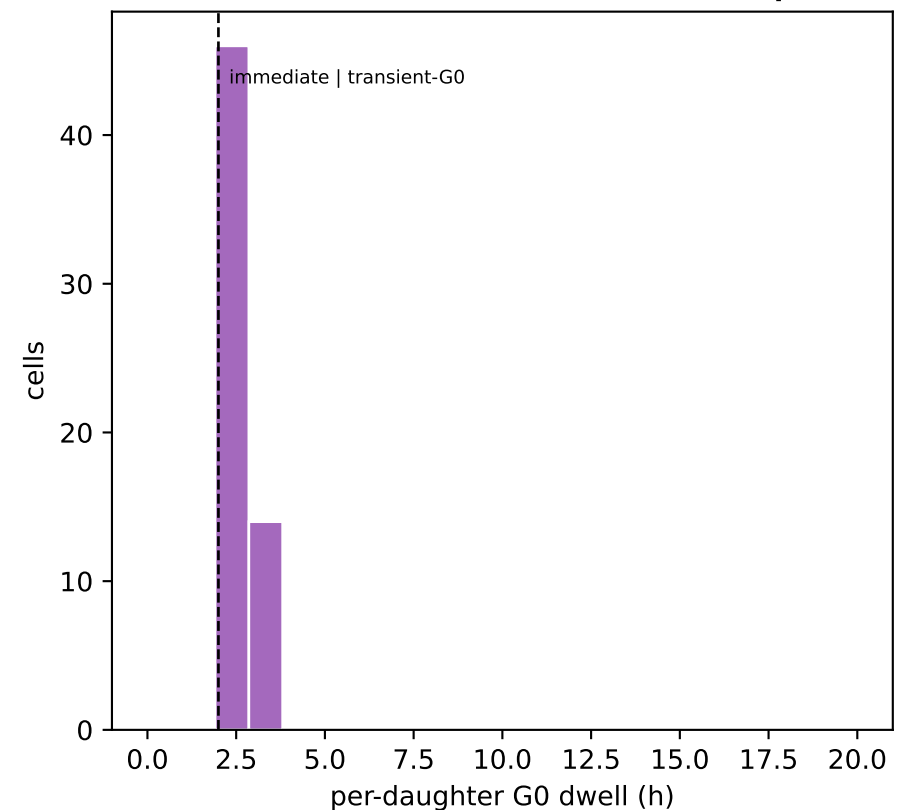
C. Dwell distribution at SHH=0.45 (the split)
