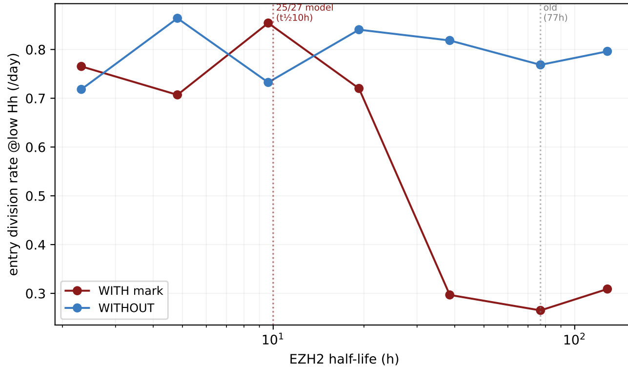
(C) MECHANISM — mark accumulates as EZH2 lives longer
