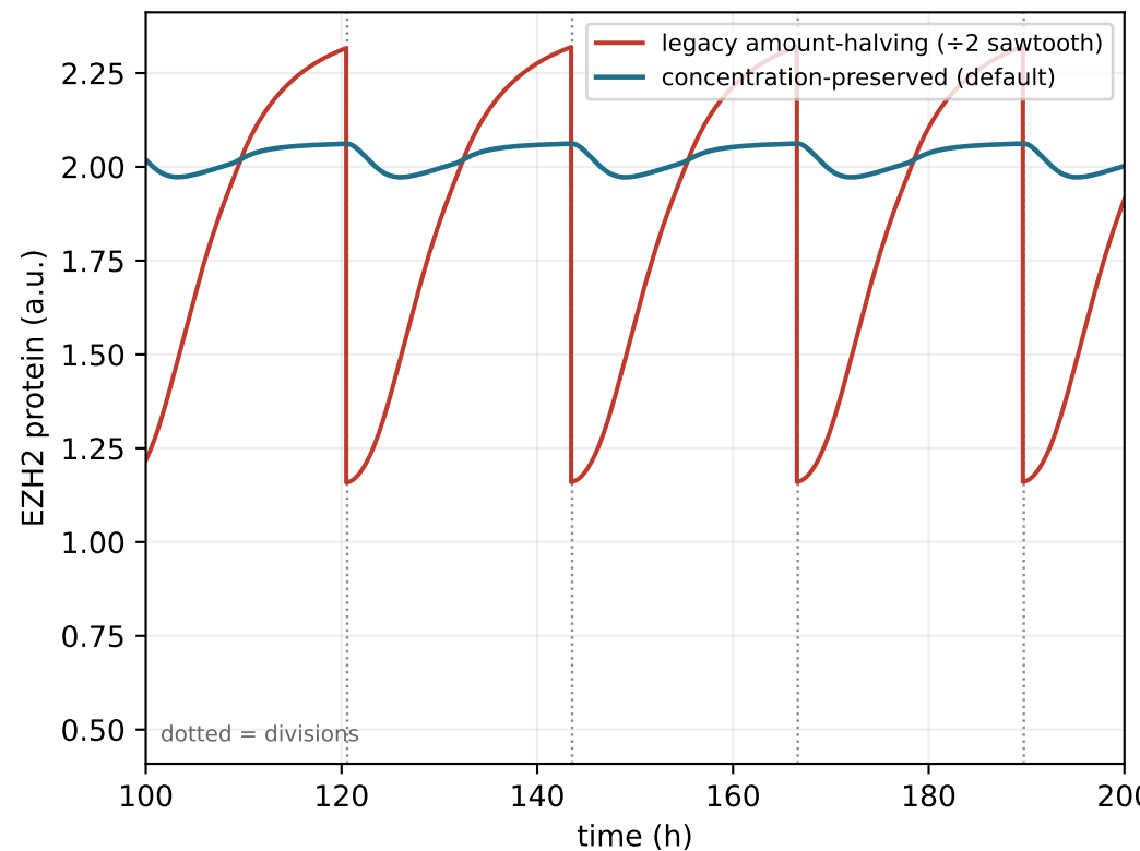
(a) EZH2 across divisions (GNP): sawtooth vs smooth
