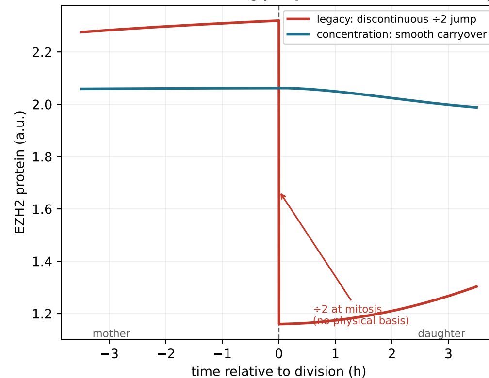
(b) One division: halving jump vs smooth ~10 h decay
