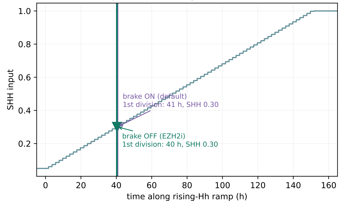
(D) Entry timing: the brake delays cell-cycle onset to higher Hh / later time
