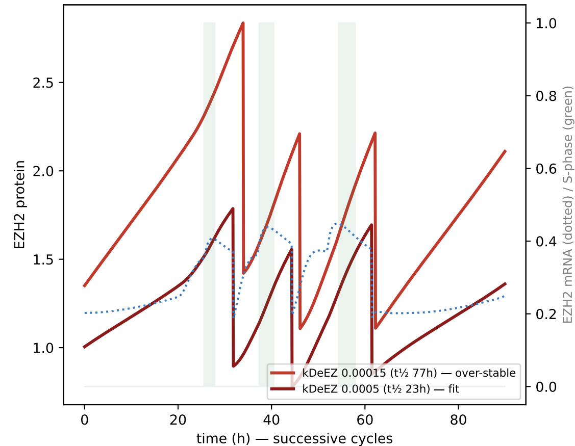
(C) EZH2 across the cell cycle (fitted baseline) rise in S → peak G2 → drop at division, on ongoing G0 baseline
