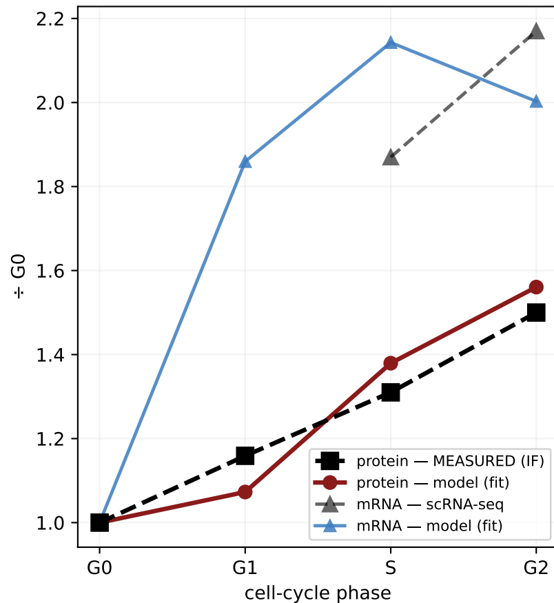
(B) Best fit: kEZbas=0.004, kDeEZ=0.0005 ( t^{1/2} 23h) protein 1.5× & mRNA ~2× both matched
