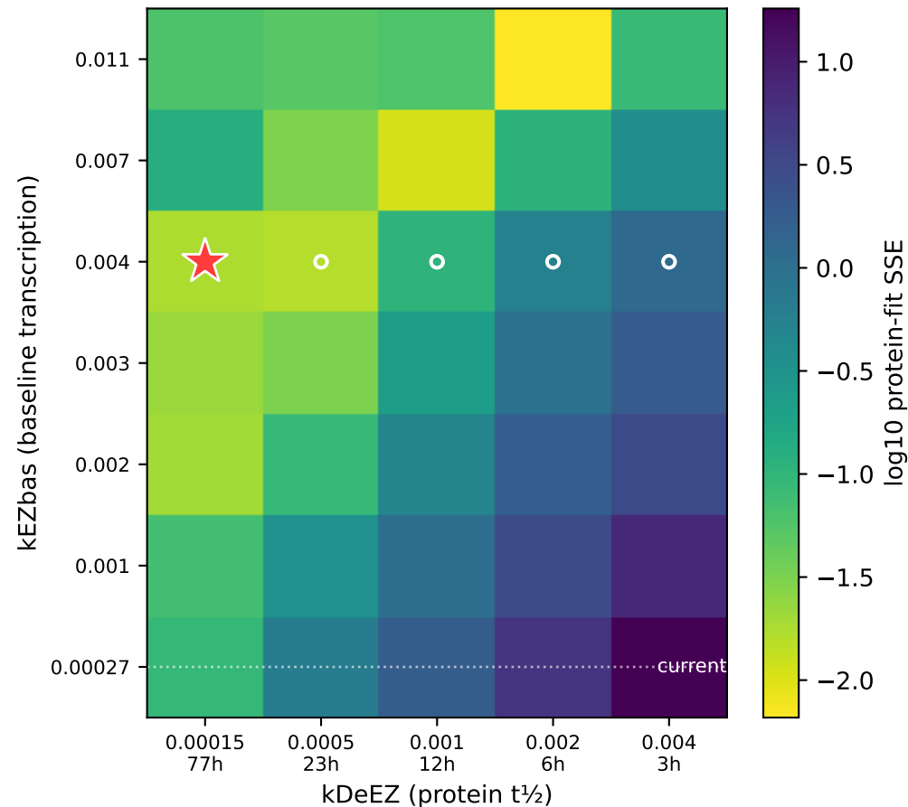
(A) Fit landscape — protein SSE ○ = mRNA also ~2× (scRNA-seq); ★ = joint best
