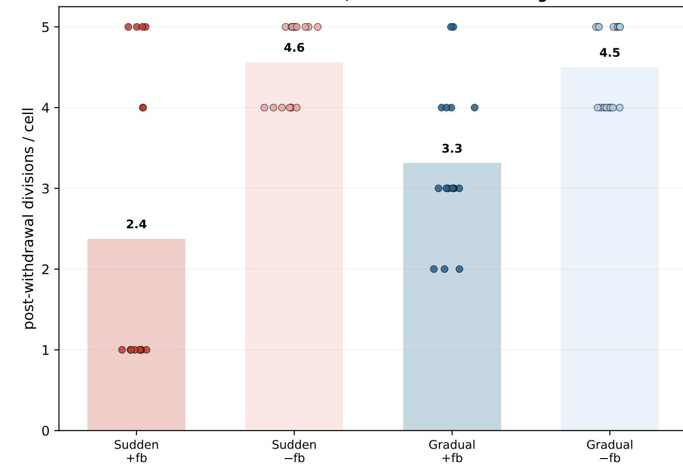
(C) Per-cell distribution at partial withdrawal (SHH→0.3) feedback → arrest; no feedback → coasting
