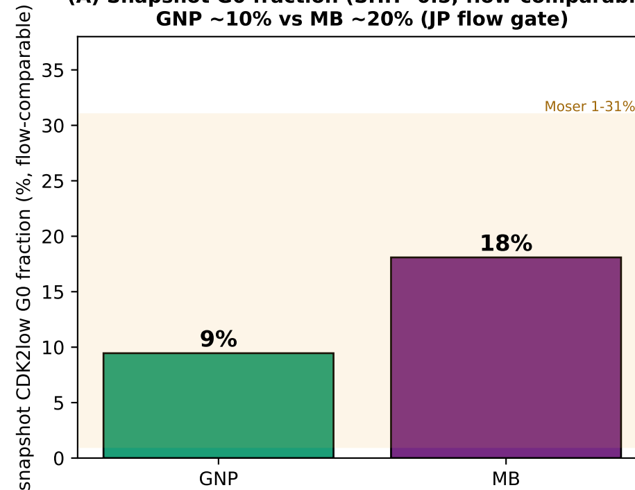
(A) Snapshot G0 fraction (SHH=0.5, flow-comparable)
