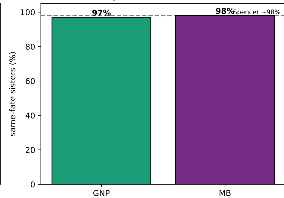
(C) Spencer sister concordance
